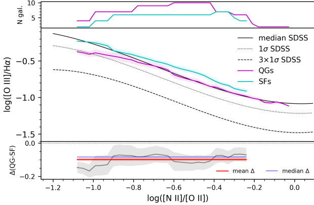
Figure 10. The average dust-corrected [\text{O III}]/\text{H}\alpha vs [\text{N II}]/[\text{O II}] diagram for the QG and SF samples. Top : the number N of galaxies that contribute to the average. Centre : The magenta curve represents the mean curve of the QG galaxies, that we obtain by averaging their means; the magenta shaded area shows the error of the average (i.e. \sigma_{\text{mean}}/\sqrt{N} ). The cyan curve shows the mean curve of the SF sample. The black curves represent median, 1\sigma and 3\times 1\sigma limit of the SDSS star-forming galaxies sample (see Q18). Bottom : the grey curve represents the differences in [\text{O III}]/\text{H}\alpha , as a function of [\text{N II}]/[\text{O II}] , between QGs and SF galaxies and the grey shaded area shows the propagated errors. The red line and pink shaded area represent the weighted mean and error of these differences averaged over the [\text{N II}]/[\text{O II}] range (see Table 2).
