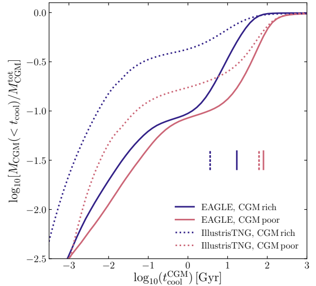
Figure 3. The cumulative distribution function of the radiative cooling times of fluid elements comprising the CGM of present-day haloes within a 0.1 dex window about M_{200} = 10^{12.5} M_{\odot} , in EAGLE (solid curves) and TNG (dotted curves). In each case, the haloes are ranked by their CGM mass fraction, f_{\text{CGM}} , and those comprising the upper and lower quartiles are stacked to form CGM-rich (blue curves) and CGM-poor (red curves) samples. Vertical lines denote the median cooling time of each stack. Despite the two simulations exhibiting significantly different CGM cooling time distributions for haloes of this mass, an aspect in common is the relative paucity of rapidly-cooling gas in the CGM-poor samples.
