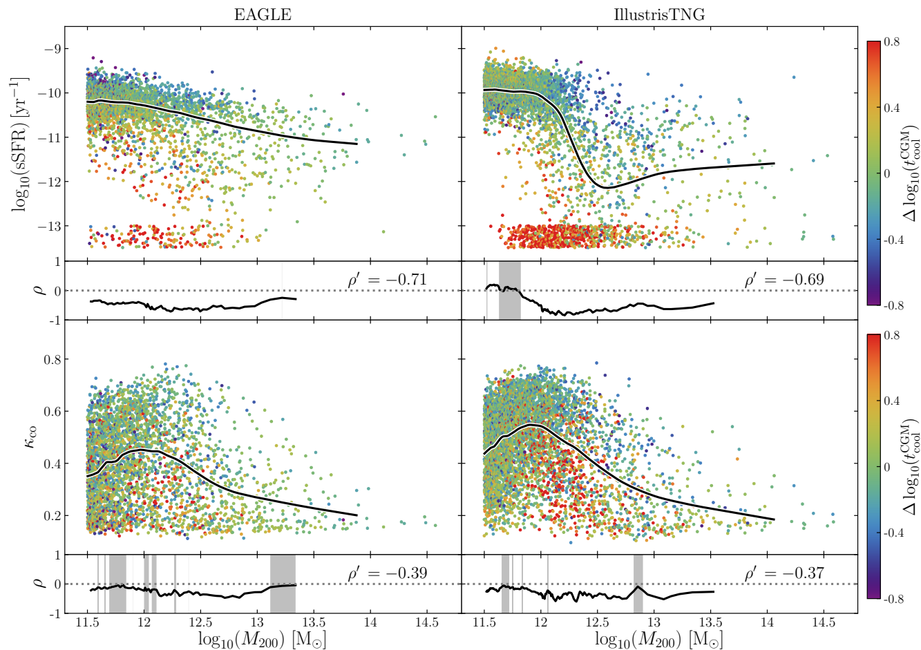
Figure 5. Present-day specific star formation rates (sSFR; upper row) and fractions of stellar kinetic energy invested in co-rotation ( \kappa_{\text{co}} ; lower row), of the central galaxies of haloes in the EAGLE (left) and TNG (right) simulations, as a function of halo mass, M_{200} . Black curves denote running medians, \text{sSFR}(M_{200}) and \kappa_{\text{co}}(M_{200}) . Symbols are coloured by residuals about the running median of the characteristic CGM radiative cooling time, t_{\text{cool}}(M_{200}) . Below each panel we show the running values of the Spearman rank correlation coefficient, \rho , of the \Delta \log_{10} \text{sSFR} versus \Delta \log_{10} t_{\text{cool}} (upper row) and \Delta \kappa_{\text{co}} versus \Delta \log_{10} t_{\text{cool}} (lower row) relations, which are shaded where the correlation has low significance ( p > 0.01 ). The quantity \rho' denotes the Spearman rank correlation coefficient for haloes within a 0.1 dex window about M_{200} = 10^{12.5} M_{\odot} . All four panels exhibit negative correlations that are significant in particular halo mass regimes, with the \Delta \log_{10} \text{sSFR} versus \Delta \log_{10} t_{\text{cool}} correlation being particularly strong at intermediate mass.
