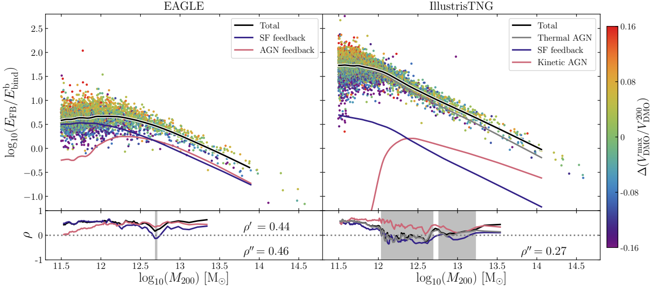
Figure 7. Present-day ratio of the total energy injected by feedback processes to the binding energy of halo baryons, E_{\text{FB}}/E_{\text{bind}}^{\text{b}} , as a function of M_{200} . Black lines correspond to the running median of this quantity considering all contributions to E_{\text{FB}} , blue lines correspond to the contribution from stellar feedback. Red lines correspond to the running median of AGN feedback in EAGLE and kinetic-mode AGN feedback in TNG, and grey lines correspond to thermal mode AGN feedback in TNG. Symbols are coloured by residuals about the running median of the quantity V_{\text{DMO}}^{\text{max}}/V_{\text{DMO}}^{200} which is a proxy for the concentration, and inner binding energy, of the halo (see text for details). Sub-panels show with black curves the running values of the Spearman rank correlation coefficient of the relations between residuals about the plotted running medians, and that denoted by the colouring. These are shaded where the correlation has low significance ( p > 0.01 ). We also show the running Spearman rank correlation coefficient if one considers the individual contributions to E_{\text{FB}} , i.e. for EAGLE E_{\text{SF}} (blue) and E_{\text{AGN}} (red) and for TNG E_{\text{SF}} (blue), E_{\text{AGN,thm}} (grey) and E_{\text{AGN,kin}} (red). The quantity \rho'' is the equivalent of \rho' = \rho(M_{200} = 10^{12.5} M_{\odot}) but considering only the main expulsive feedback mode in each simulation, i.e. AGN feedback in EAGLE and kinetic-mode AGN feedback in TNG.
