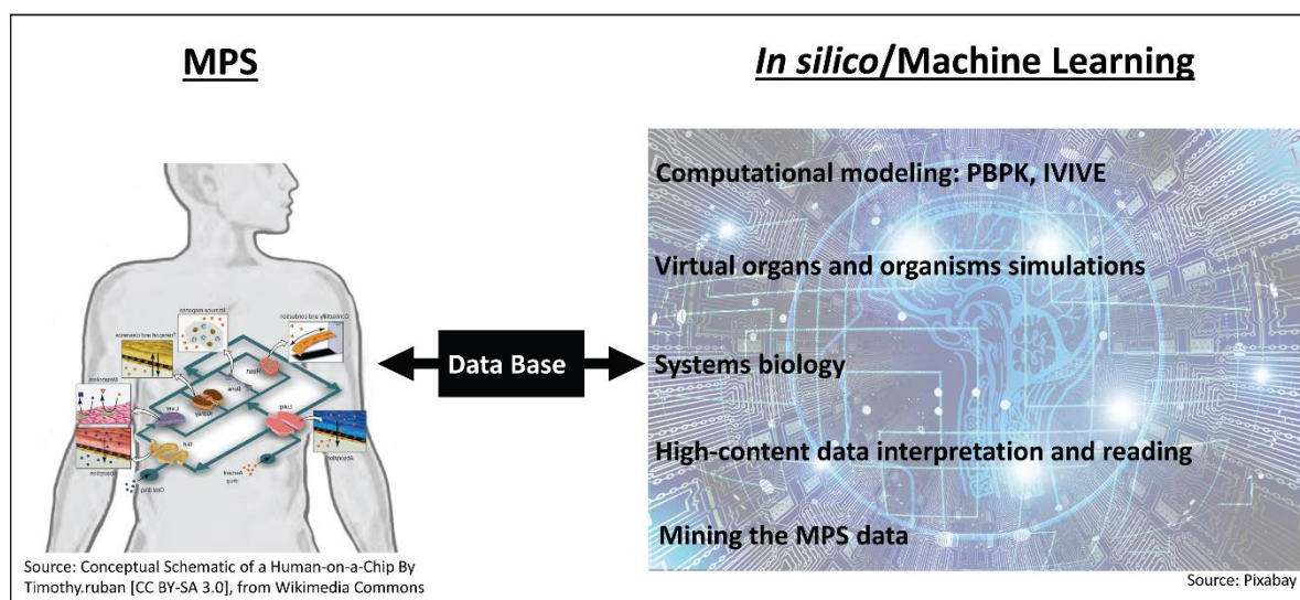
Fig. 12: Schematic illustration of merging technologies of MPS and machine learning to continuously improve in vitro and in silico models towards the systemic organismal emulation of human (patho)biology (adopted from Smirnova et al., 2018).
