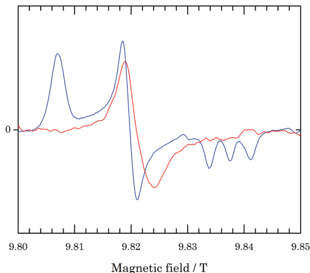
Fig. 2 275 GHz cw EPR spectra of TEMPOL (1 mM) in water and glycerol 1 : 1 in volume at a cryostat temperature of -47\text{ }^\circ\text{C} . The spectrum in red is taken under continuous laser irradiation at a nominal power of 3.5 W, which increases the temperature of the sample to 5\text{ }^\circ\text{C} .
