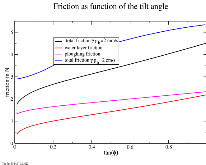
Figure 5: The friction contributions as function of the tilt angle
