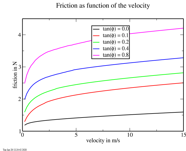
Figure 6: The friction as function of the velocity for various tilt angles
