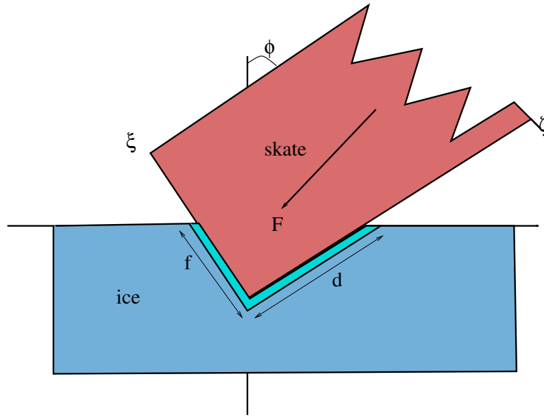
Figure 2: Tilted Skate indenting the Ice
