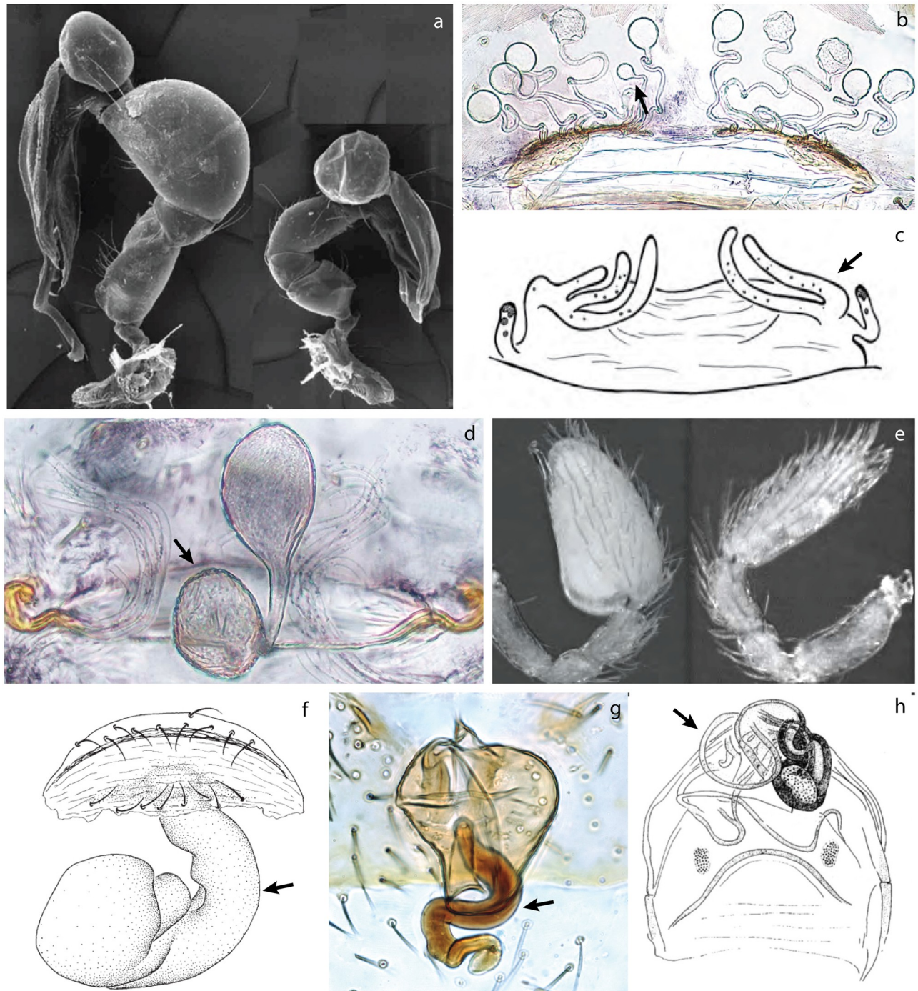
Fig 2. Examples of genital asymmetry in Synspermiata. a, e) male pedipalps, lateral view. b–d, f–h) vulva, dorsal view. a) Pholcidae: Metagonia mariquitarensis ; modified from Huber [9]. b) Ochyroceratidae: Altheopus naphongensis ; modified from Li et al. [18]. c) Sicariidae: Hexophthalma albospinosa ; modified from Magalhaes and Brescovit [19]. d) Ochyroceratidae: Speocera cattien ; modified from Tong, et al. [20]. e) Oonopidae: Paradysderina rightly ; modified from Platnick and Dupérré [21]. f) Telemidae: Telema exiloculata ; modified from Lin and Li [22]. g) Oonopidae: Triaeris stenaspis . h) Pholcidae: Metagonia delicata ; modified from Huber [23]. Arrows indicate the asymmetric structure: b, c: number and development of spermathecae. d: size of spermathecae. f–g: direction of seminal receptacle.
