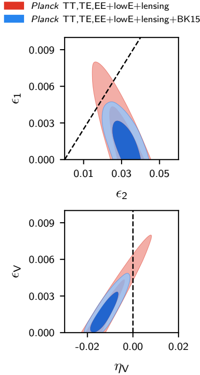
Fig. 6. Marginalized joint two-dimensional 68% and 95% CL regions for (\epsilon_1, \epsilon_2) (top panel) and (\epsilon_V, \eta_V) (bottom panel) for Planck TT,TE,EE+lowE+lensing (red contours), compared with Planck TT,TE,EE+lowE+lensing+BK15 (blue contours). The dashed lines divide between convex and concave potentials.
