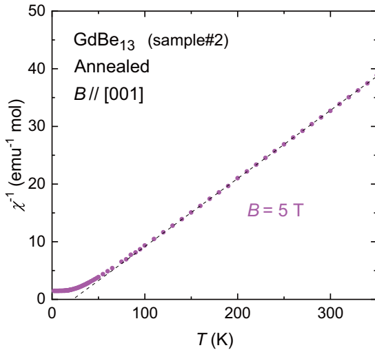
FIG. 5. Temperature dependence of the inverse magnetic susceptibility \chi^{-1}(T) [ = B/M(T) ] of \text{GdBe}_{13} for the annealed sample 2 at B = 5 T applied along [001]. The dashed line represents a CW fit in the temperature range between 150 and 350 K.
