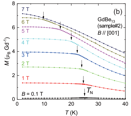
FIG. 6. (a) Temperature dependence of the magnetic susceptibility \chi(T) [ = M(T)/B ] for \text{GdBe}_{13} below 50 K at B = 0.1 T applied along [001]. The open and closed symbols represent the data upon ZFC and FC processes, respectively. The inset shows d\chi/dT as a function of T at 0.1 T. (b) Temperature dependence of the magnetization M(T) at several fields up to 7 T for B \parallel [001] .
