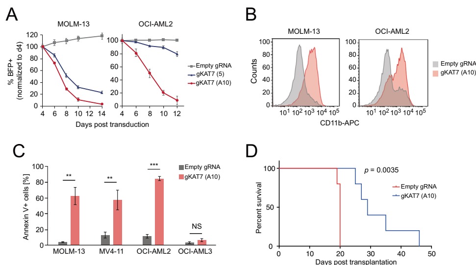
Fig. 1 Loss of KAT7 exhibits antileukemic effects in vitro and in vivo. a Proliferation of KAT7 KO using two sgRNAs or empty control in MLL-X AML cell lines. Percentages of BFP-positive ( KAT7 -KO) cells were assayed at the indicated time point and were normalized to day 4. Data are shown as mean \pm SD ( n = 3 ). b CD11b staining in WT (empty gRNA) and KAT7 KO (gKAT7-A10) cells 7 days post
