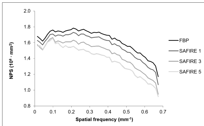
Figure 5. Noise power spectra at 120 kV D. Noise power spectra at 120 kV for FBP, SAFIRE 1, 3 and 5, the profile was the same for all other tube potentials. Published with permission from Acta Radiologica.
