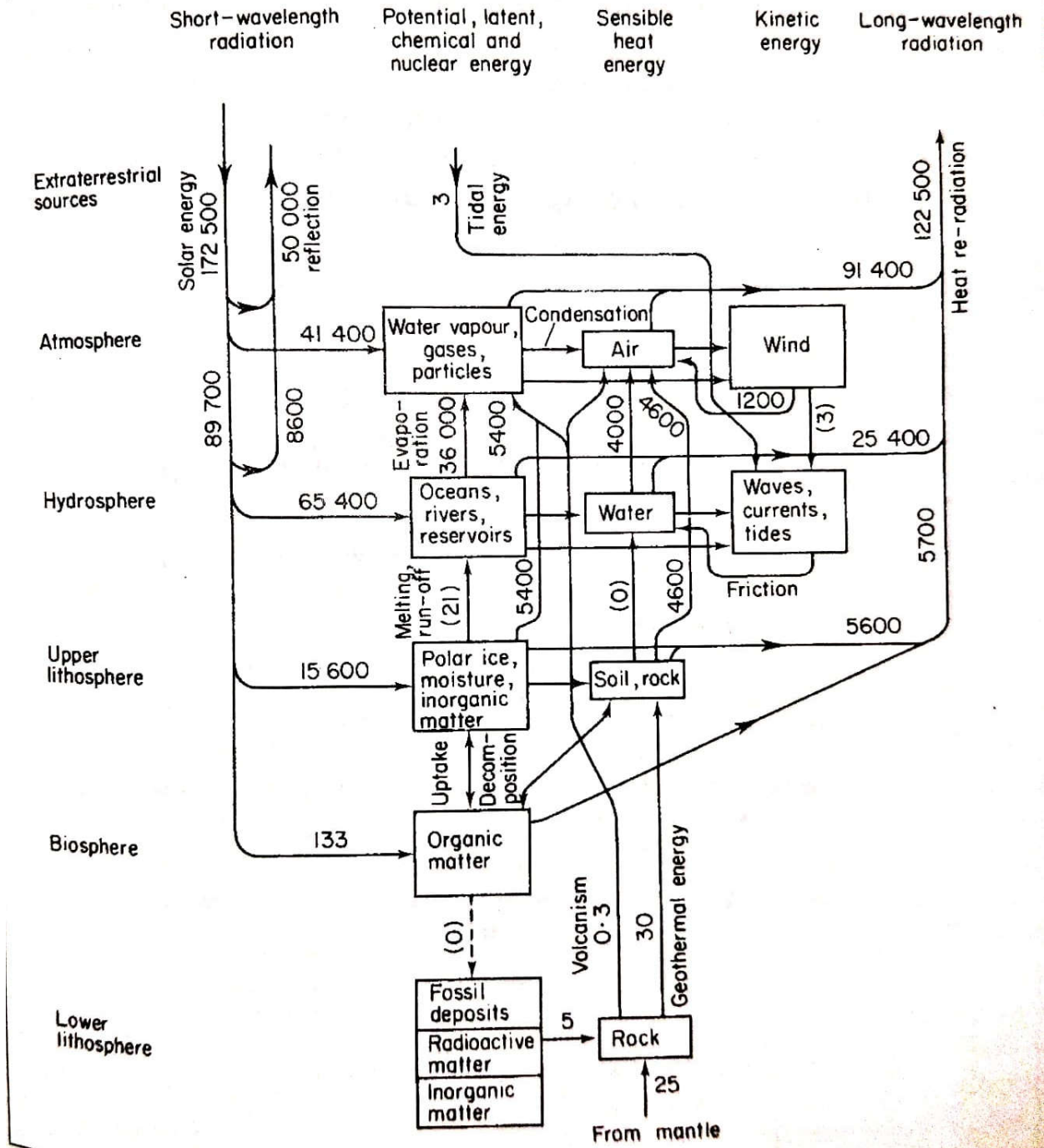
Figure 1.2: Schematic energy cycle without anthropogenic interference [4].
