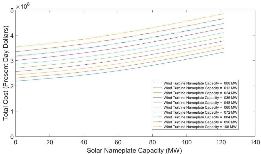
Figure 4.29: Yearly net present cost of energy for different sizes of combined wind and solar installations located in Dallas, Texas using $1950 per kW nameplate capacity for wind, $1500 per kW nameplate capacity for solar, an industrial electricity price of $0.0557 per kW-h for purchasing electricity to cover energy deficits.
