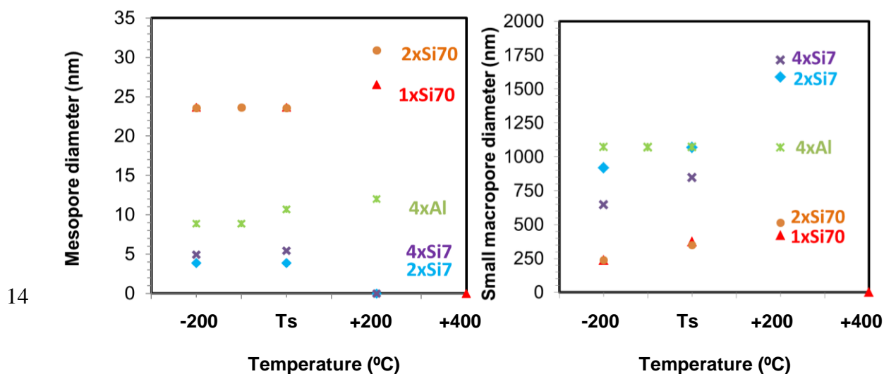
14 15 16 Figure SI4. Porosity created in the SiCfs monolith by infiltration with the different colloidal metal oxide solutions as 17 a function of the calcination temperature. Left: Size of the pores created by the oxide interparticular voids. Right: 18 Size of the small macropores created by neck size reduction.
