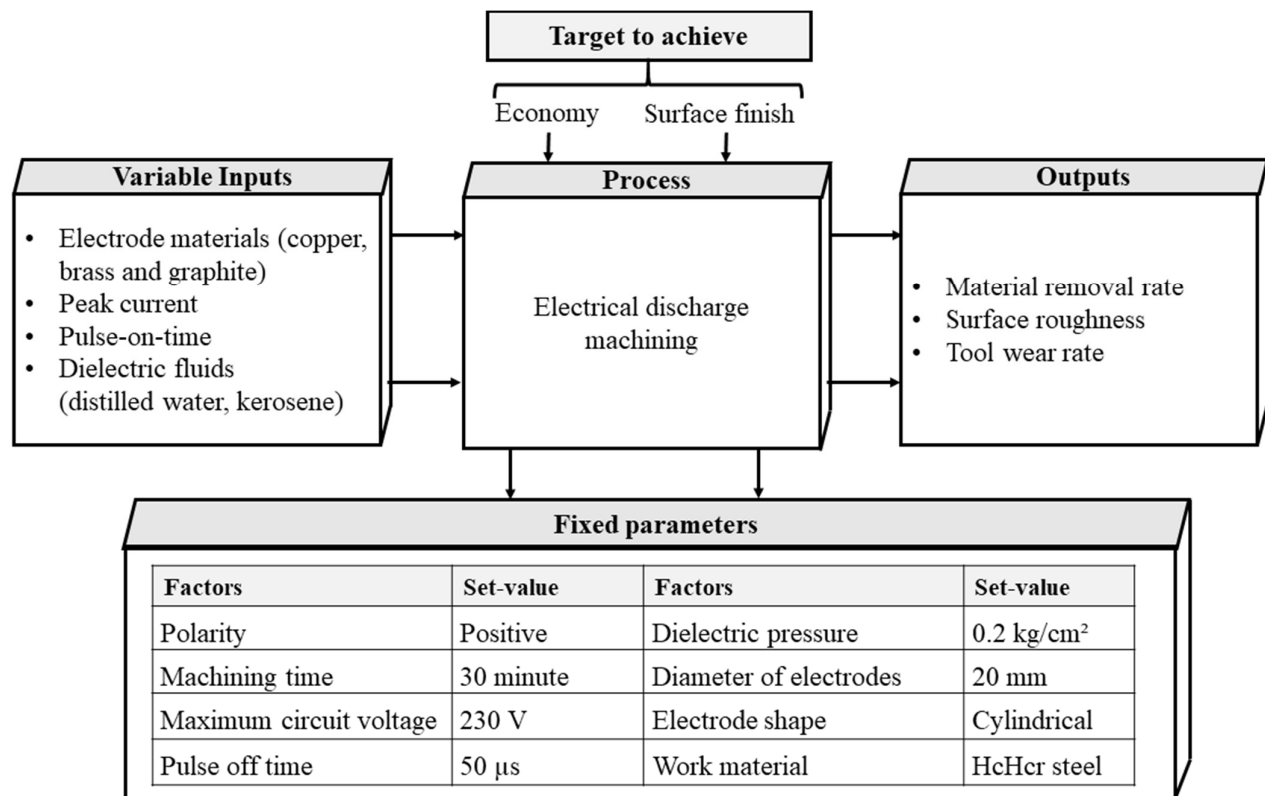
Figure 3. Experimental input-output model of EDM process.
