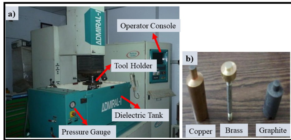
Figure 2. (a) Electrical discharge machining (EDM) experimental setup; (b) tools for experimentation.
