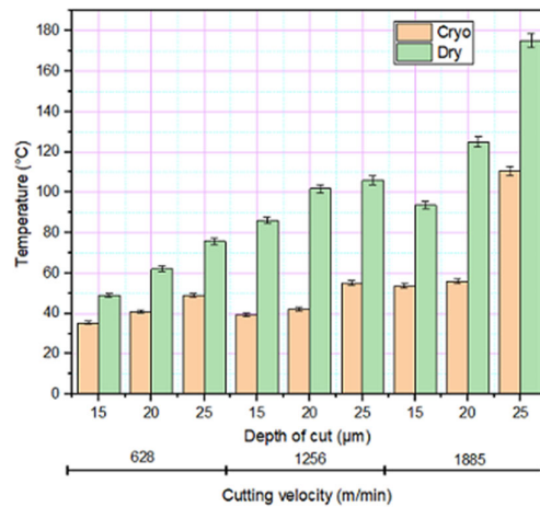
Figure 3. Variation in temperature under different grinding environments.
