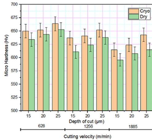
Figure 6. Variation of microhardness at different grinding environments.
