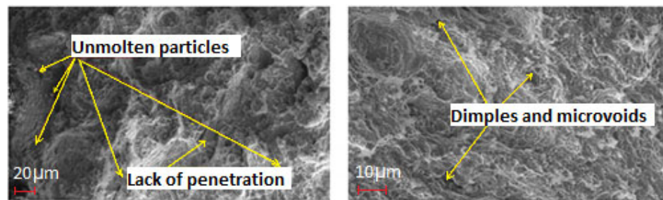
Figure 12. Fractographic analysis of samples.
