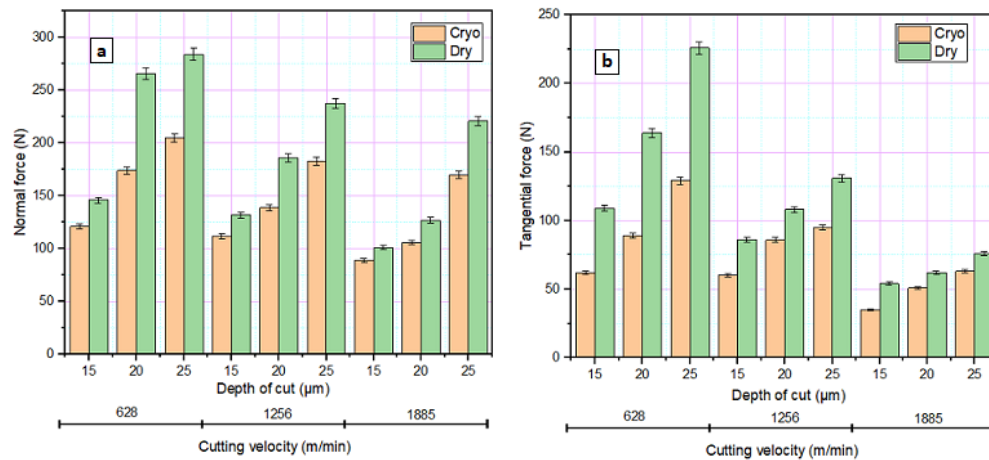
Figure 2. Variation in grinding force under different grinding environments. (a) Normal force and (b) Tangential force.
