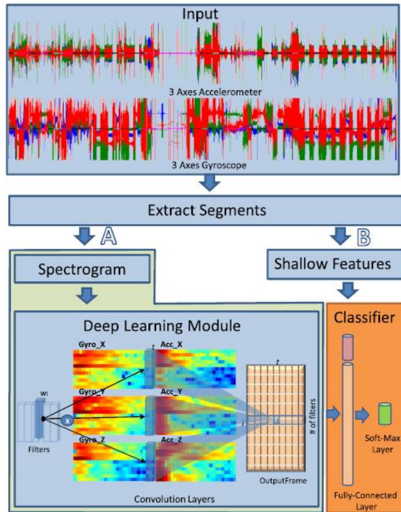
Figure 4.1 Deep learning module.
