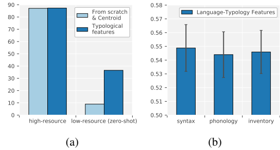
Figure 4: (a) Impact of language typology features on parsing performance (LAS). (b) Average of normalized feature weights obtained from linear projection layer of the language embedding network.
