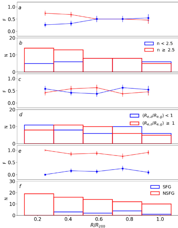
Figure 11. The fraction (F) and histogram representing the number of galaxies (N) per R_{200} bin. Panels a and b show galaxies with n_r \geq 2.5 and < 2.5 in red and blue, respectively. Panels c and d show galaxies with (R_{e,z}/R_{e,g}) \geq 1 and < 1 in red and blue respectively, finally panels e and f show NSFG and SFG in red and blue, respectively.
