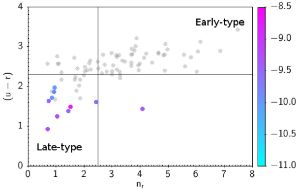
Figure 9. Same as Fig. 8, but colour-coded by the \log(sSFR) . The grey dots are NSFG.
