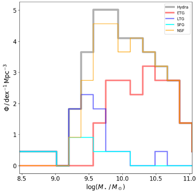
Figure 6. Stellar mass function of galaxies brighter than m_r=16 within a sphere with 1.4 Mpc of radius centred on Hydra. The grey line is the 81 galaxies belonging to Hydra selected as indicated in subsection 2.1. The orange and cyan lines are the quenched (NSFGs) and SFGs. The red and blue lines are ETGs and LTGs, respectively.
