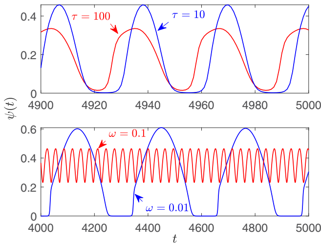
FIG. 13. Steady state oscillations of \psi(t) calculated from Eqs. (8) and (9) at T = 0.9T_c with q = q_a \sin \omega t for different \tau at \omega = 0.1 and q_a = 1.35 (top) and different \omega at \tau = 100 and q_a = 1.30 (bottom).
