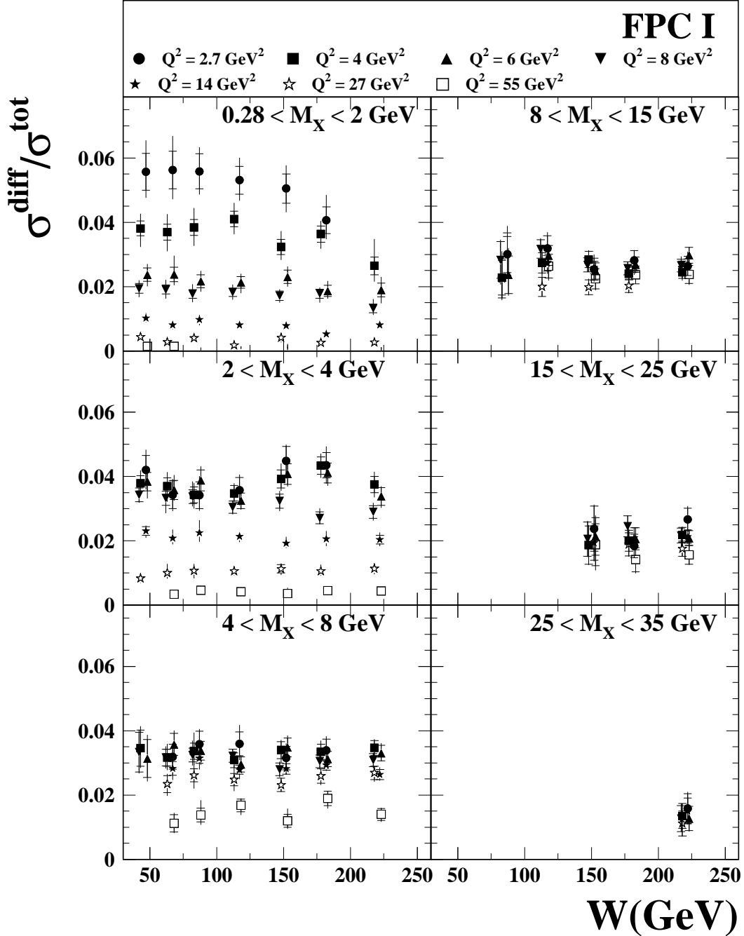
Figure 16: The ratio of the diffractive cross section, integrated over the M_X intervals indicated, \int_{M_a}^{M_b} dM_X d\sigma_{\gamma^*p \rightarrow XN, M_N < 2.3\text{GeV}}^{\text{diff}}/dM_X , to the total \gamma^*p cross section, r_{\text{tot}}^{\text{diff}} = \sigma^{\text{diff}}/\sigma_{\gamma^*p}^{\text{tot}} , as a function of W for the Q^2 intervals indicated. The inner error bars show the statistical uncertainties and the full bars the statistical and systematic uncertainties added in quadrature. The plot shown is taken directly from the FPC I paper.
