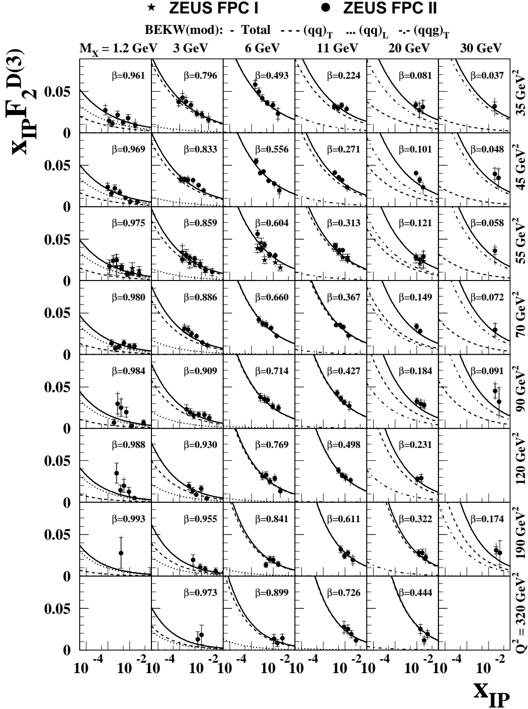
Figure 20: The diffractive structure function of the proton multiplied by x_{\mathbb{P}} , x_{\mathbb{P}} F_2^{D(3)} , for \gamma^* p \rightarrow XN , M_N < 2.3 \text{ GeV} as a function of x_{\mathbb{P}} for different regions of \beta and Q^2 \geq 35 \text{ GeV}^2 : both FPC I data (stars) and FPC II data (dots) are shown. The inner error bars show the statistical uncertainties and the full bars the statistical and systematic uncertainties added in quadrature. The curves show the results of the BEKW(mod) fit for the contributions from (q\bar{q}) for transverse (dashed) and longitudinal photons (dotted) and for the (q\bar{q}g) contribution for transverse photons (dashed-dotted) together with the sum of all contributions (solid). For display purposes, some of the x_{\mathbb{P}} F_2^{D(3)} values at Q^2 = 90, 120, 190 and 320 \text{ GeV}^2 with large uncertainties are not shown but given in Tables 27 – 29.
