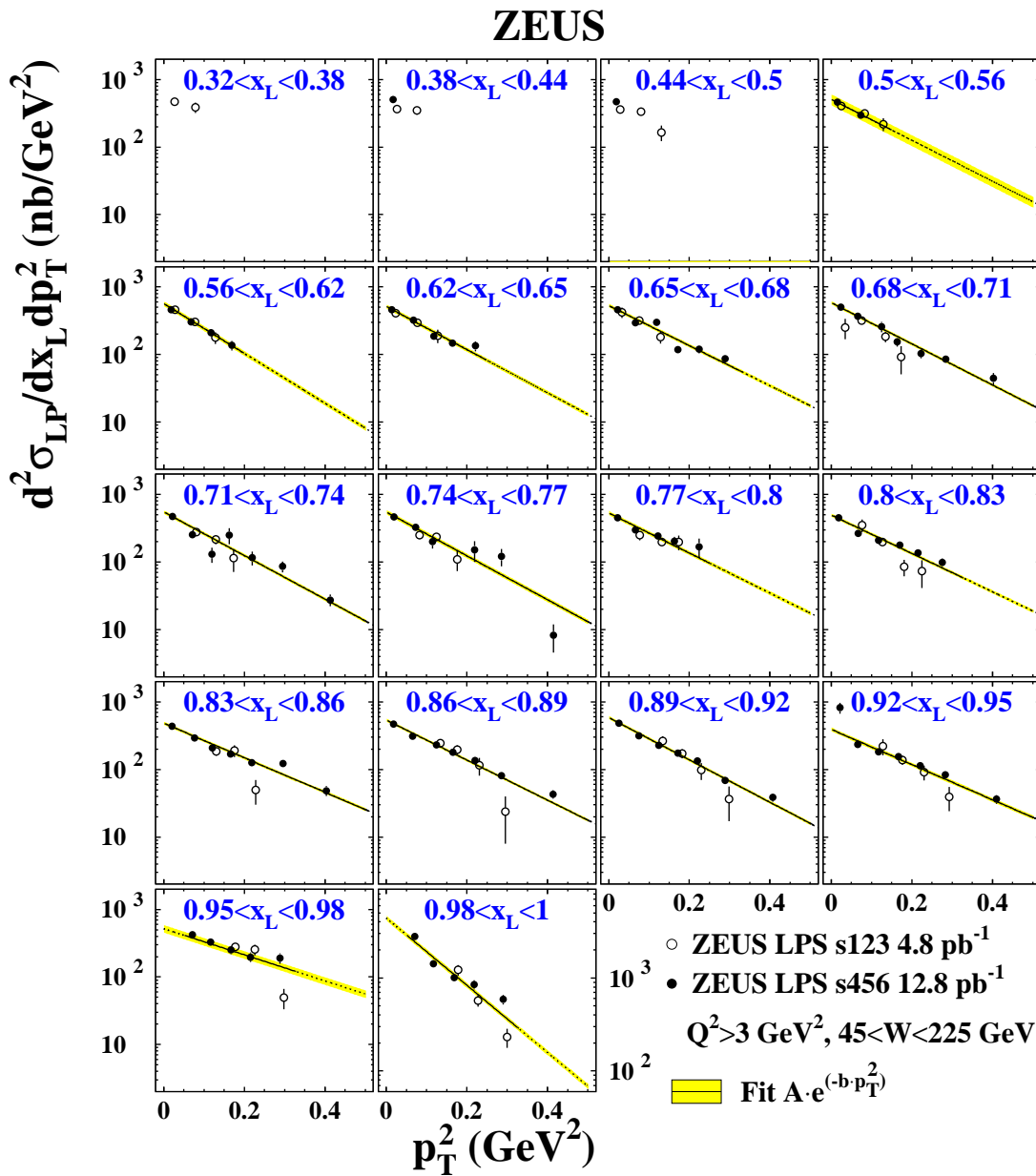
Figure 6. The double-differential cross-section d^2\sigma_{LP}/dx_L dp_T^2 for Q^2 > 3 \text{ GeV}^2 and 45 < W < 225 \text{ GeV} as a function of p_T^2 in bins of x_L . The circles and the dots are the ZEUS data measured with the spectrometers s123 and s456, respectively. For clarity, only the statistical uncertainties are shown. The systematic uncertainties are listed in table 1. The lines are the result of a fit to a function A \cdot e^{-b \cdot p_T^2} , as described in the text. The solid lines indicate the range in which the fit was performed. The bands show the statistical uncertainty of the fit.
