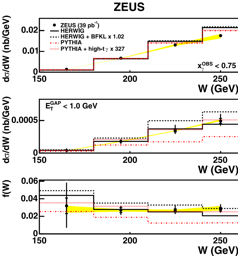
Fig. 12. The top plot is the inclusive dijet cross section for x_\gamma^{\text{OBS}} < 0.75 differential in W , the middle plot is the corresponding gap cross section differential in W requiring that E_T^{\text{GAP}} < 1 GeV, and the bottom plot is the gap fraction, f , as a function of W . Other details as in Fig. 1
