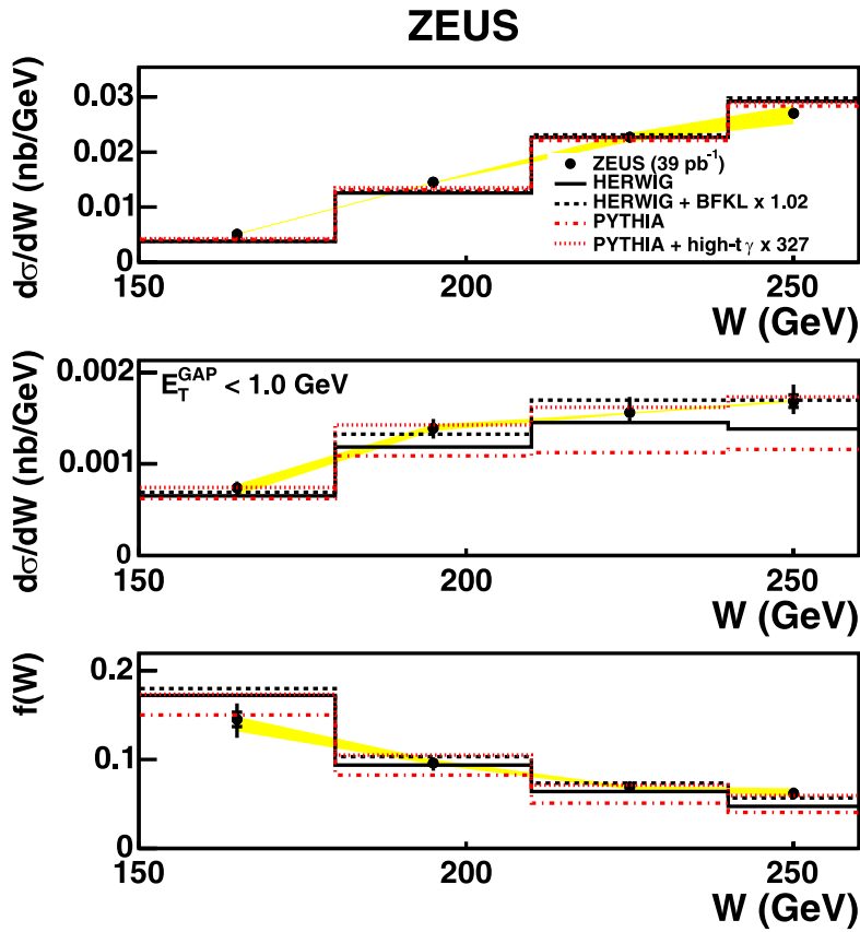
Fig. 8. The top plot is the inclusive dijet cross section differential in W , the middle plot is the gap cross section differential as a function of W requiring that E_T^{\text{GAP}} < 1.0 GeV, and the bottom plot is the gap fraction, f , as a function of W . Other details as in Fig. 1
