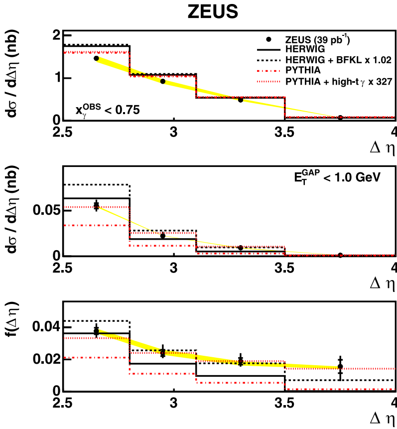
Fig. 10. The top plot is the inclusive dijet cross section for x_\gamma^{\text{OBS}} < 0.75 differential in \Delta\eta , the middle plot is the corresponding gap cross section differential in \Delta\eta requiring that E_T^{\text{GAP}} < 1 GeV, and the bottom plot is the gap fraction, f , as a function of \Delta\eta . Other details as in Fig. 1
