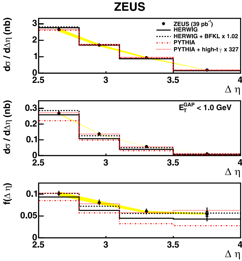
Fig. 2. The top plot is the inclusive dijet cross section differential in \Delta\eta , the middle plot is the gap cross section differential in \Delta\eta requiring that E_T^{\text{GAP}} < 1 GeV, and the bottom plot is the gap fraction, f , as a function of \Delta\eta . Other details as in Fig. 1
