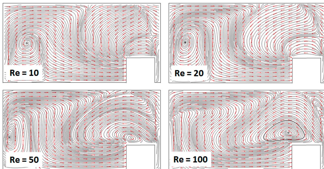
Figure 8. Cross-sectional streamline/arrow plots of the velocity field for the mixer with R_{in} = 400 \mu\text{m} , at different Reynolds numbers. The data is collected midway through the second mixing subsection.
