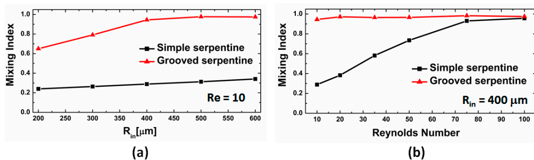
Figure 7. (a) Dependence of the mixing index on the radius of curvature R_{in} at Re = 10 ; (b) Dependence of the mixing index on the Reynolds number for the design with R_{in} = 400 \mu\text{m} .
