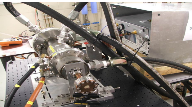
Fig. 1. A photo of the W-band gyro-TWA.
