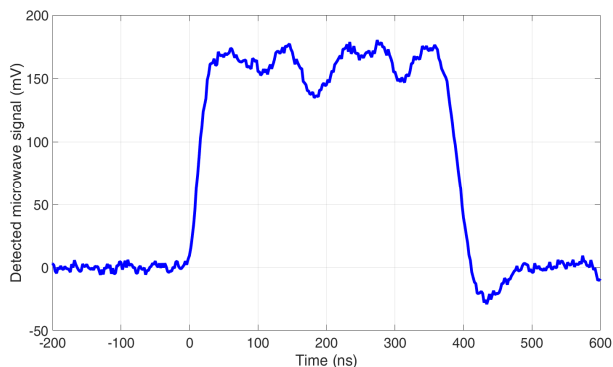
Fig 3. A typical microwave pulse output from the gyro-TWA.
