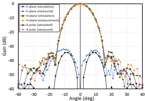
Fig 2. The measured and simulated co-polar E-plane, H-plane and cross-polar D-plane scans of the output coupler with window at 94 GHz.
