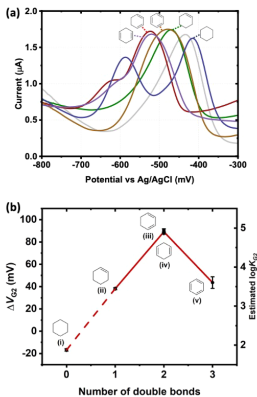
Figure 3. (a) Square wave voltammetric response of CB8- \text{MV}^{2+} -G2 ternary complexes and CB8- \text{MV}^{2+} (gray). G2 = (i) cyclohexane (blue), (ii) cyclohexene (green), (iii) 1,3-cyclohexadiene (red), (iv) 1,4-cyclohexadiene (purple) and (v) benzene (brown); (b) Plot of \Delta V_{\text{G2}} and the estimated \log K_{\text{G2}} of CB8- \text{MV}^{2+} -G2 complexes against number of double bonds in G2.
