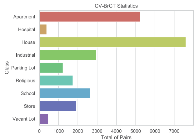
Fig. 3. Class distribution of the proposed CV-BrCT dataset.
