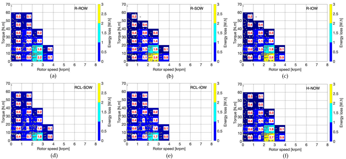
Figure 12. Energy loss distributions of the IPMSM with (a) R-ROW, (b) R-SOW, (c) R-IOW, (d) RCL-SOW, (e) RCL-IOW, and (f) H-NOW arrangements, along the ARTEMIS urban driving cycle.
