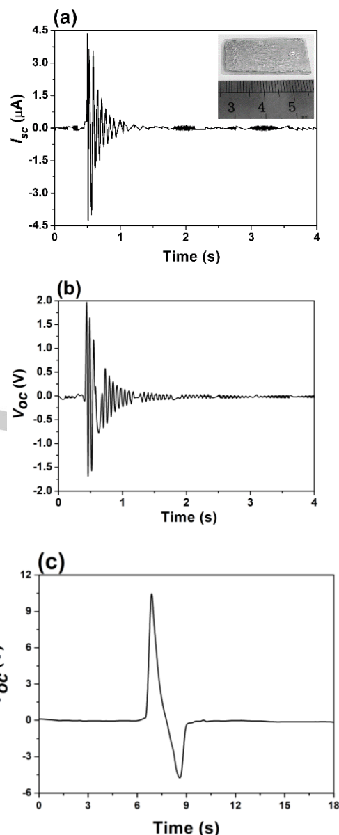
Figure 4 Piezoelectric sensing response via mechanical excitation with the output of (a) short-circuit current; (b) open circuit voltage. (c) Piezoelectric sensing performance via finger tapping with the output of open circuit voltage. While Figure 3c, demonstrates the material as a pyroelectric device, Figure 4 demonstrates its ability to operate as a piezoelectric sensor when subjected to mechanical oscillation. The material was bonded to a cantilever beam (Figure S11) which was subjected to a mechanical impulse to oscillate the beam leading to vibration which gradually decayed with time due to damping. As can be seen from Figures 4a and 4b, a 4.46 \mu\text{A} short-circuit current and 1.98 \text{ V} open-circuit voltage were initially generated, and both the current and voltage decreased as the vibration of the cantilever subsequently decayed with time. When the poled material was used as a stand-alone sensor and was subjected to a single mechanical impact by a finger, as shown in the inset of Figure S12, a positive polarity short circuit current ( -0.42 \mu\text{A} , Figure S12) and open circuit voltage ( -10.85 \text{ V} , Figure 3c) were detected which was followed by current and voltage of opposing polarity as the pressure was released and compensation charges flowed in the opposite direction.
