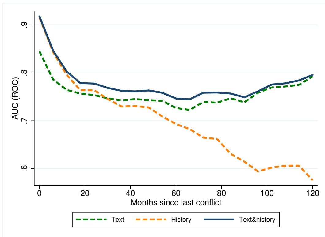
Fig. 4: AUC scores with fading conflict history
