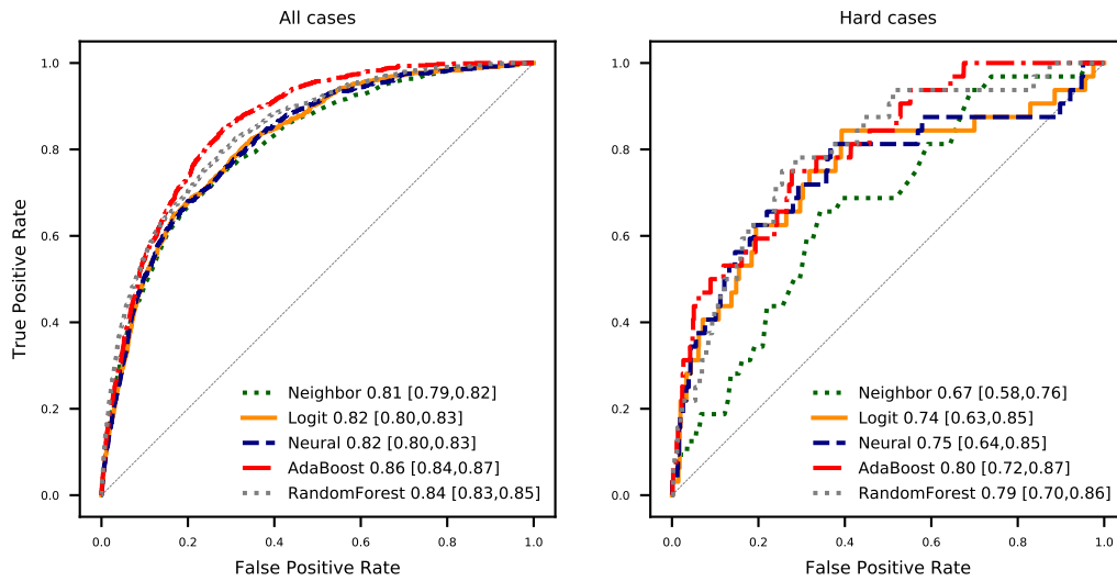
Fig. E.9: ROC curves of forecasting violence with different algorithms using only text
