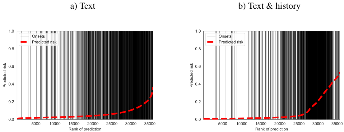
Fig. E.8: Separation plot of forecasting any violence using text and conflict history
