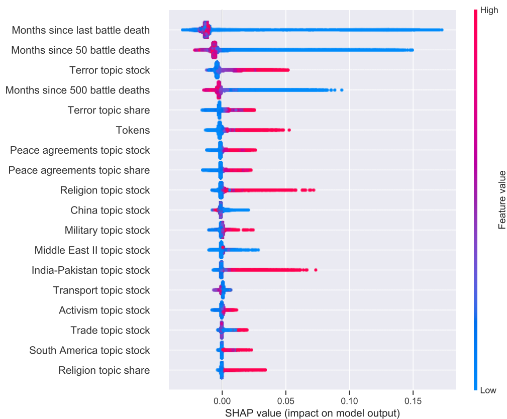
Fig. 8: SHAP beeswarm plots of predictors
