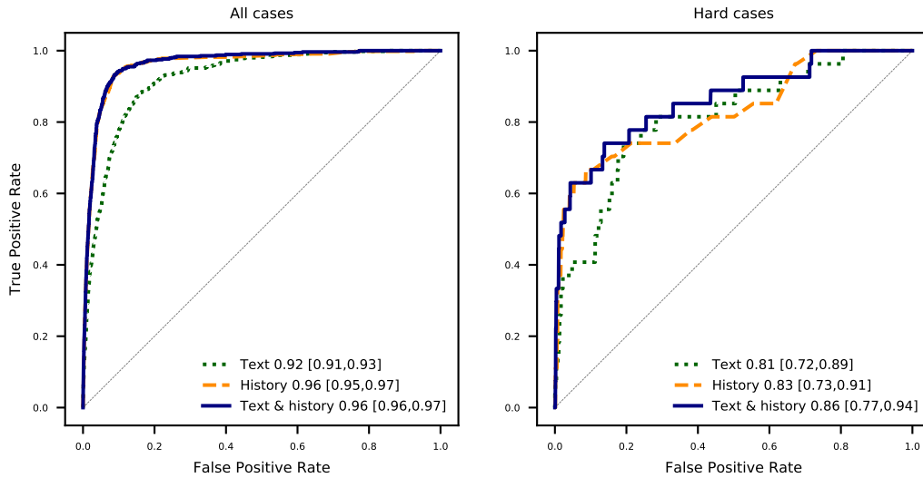
Fig. E.7: ROC curves of forecasting armed conflict with at least 50 battle deaths
