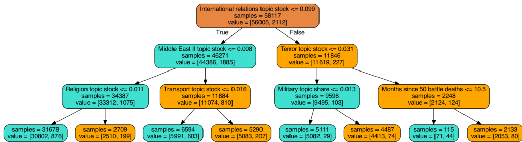
Fig. 6: Simplified example tree of depth 3
