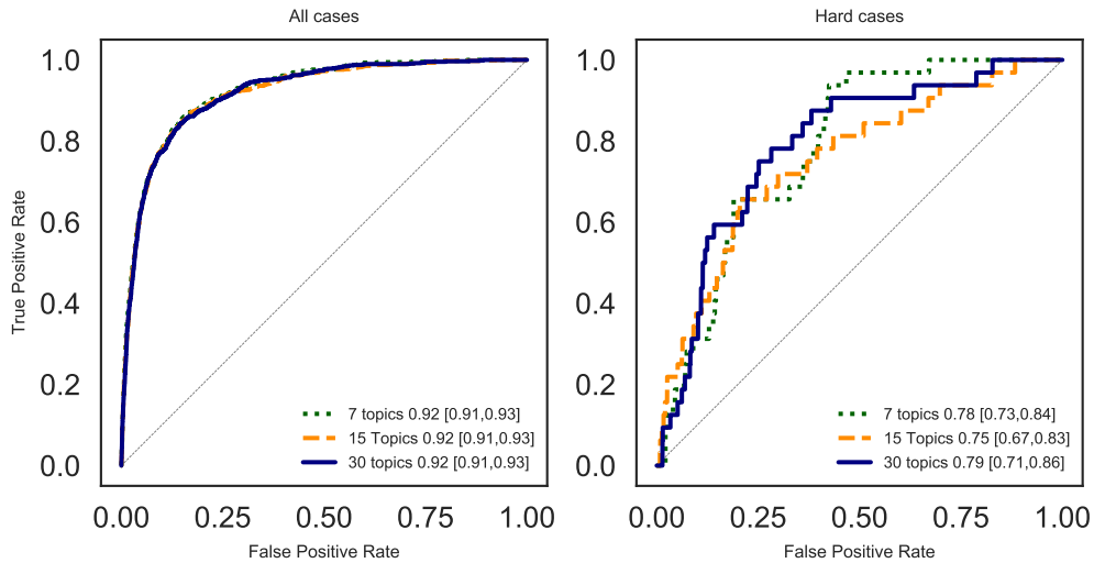
Fig. E.6: ROC curves of forecasting violence with varying number of topics using text and history
