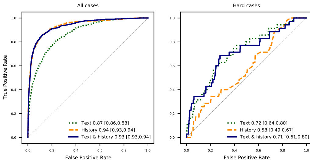
Fig. E.1: ROC curves for predictions of onset within next quarter
