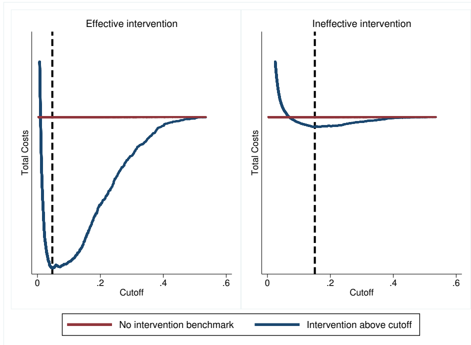
Fig. 9: Cost curves with effective and ineffective interventions
