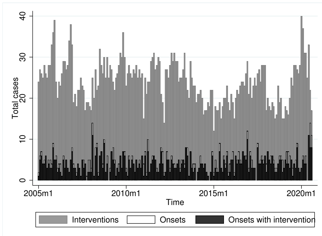
Fig. D.1: Simulating timing and frequencies of effective interventions
