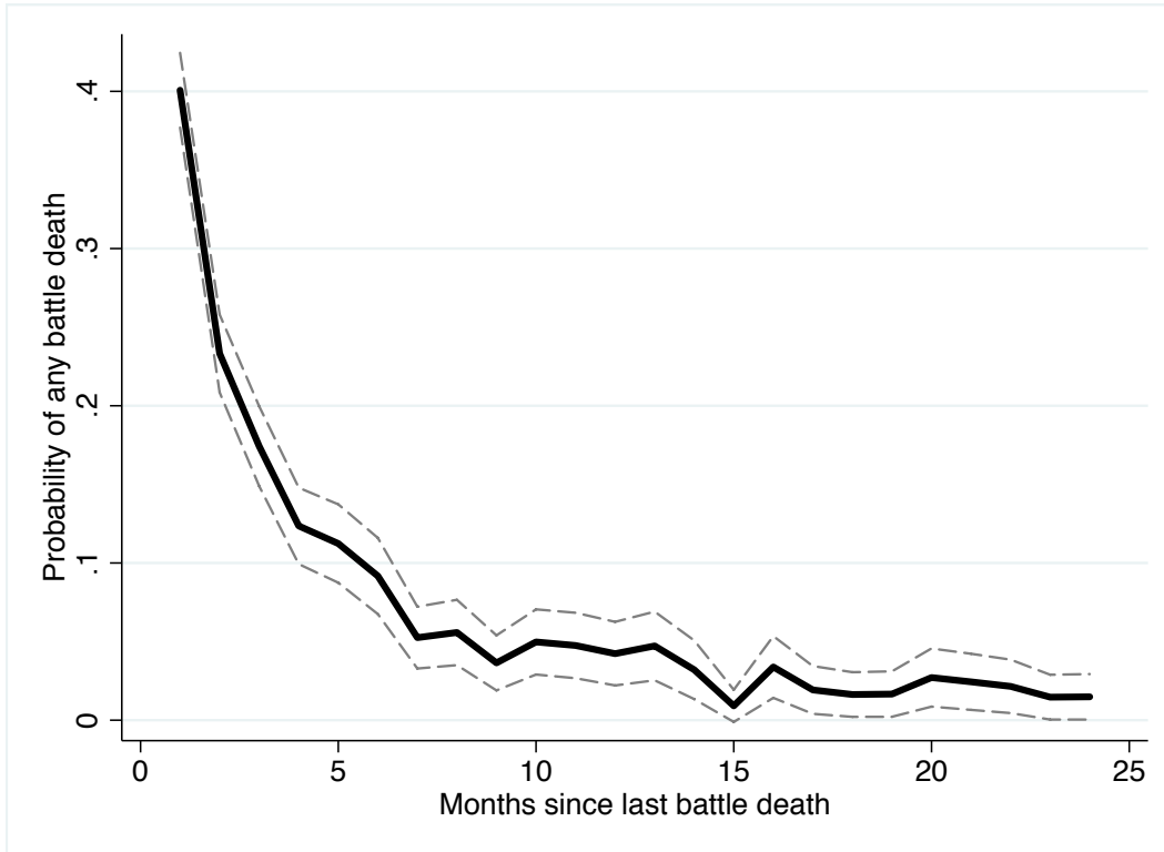
Fig. 1: Likelihood of conflict relapse post conflict
