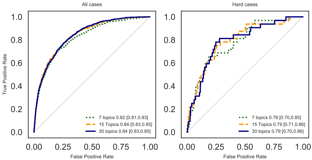
Fig. E.5: ROC curves of forecasting violence with varying number of topics using only text
