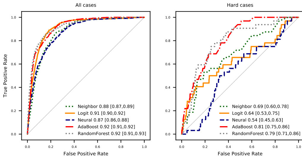
Fig. E.10: ROC curves of forecasting violence with different algorithms using text and history
