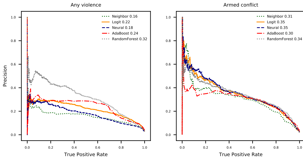
Fig. E.11: Precision curves of forecasting violence with different algorithms using text and history
