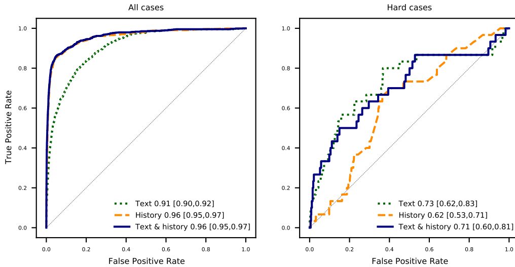
Fig. E.2: ROC curves for predictions of onset within next year
