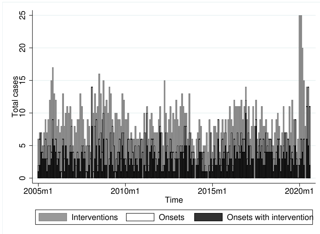
Fig. D.2: Simulating timing and frequencies of ineffective interventions
