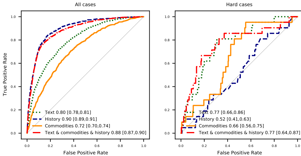
Fig. E.4: ROC curves of forecasting any violence (left) and armed conflict (right) compared to commodity prices
