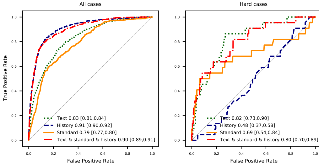
Fig. E.3: ROC curves of forecasting any violence (left) and armed conflict (right) compared to standard variables
