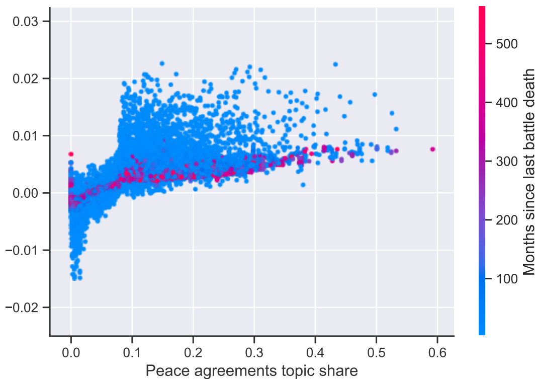
Fig. C.4: SHAP values of all individual predictors depending on time since last battle death
