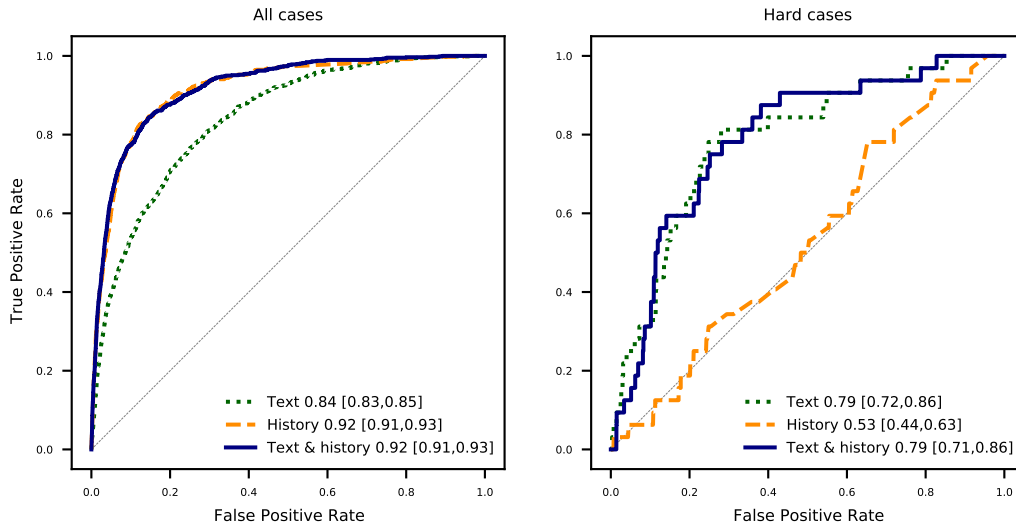
Fig. 3: ROC curves of forecasting any violence for all cases (left) and hard cases (right)
