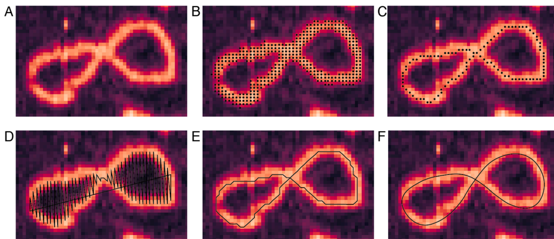
Fig. 2. Representative image sequence showing the steps in the tracing process for an individual DNA minicircle. (A) The original topographical image of a DNA minicircle. (B) The automatically generated Gwyddion grain (shown as black dots) overlaid on the DNA molecule. (C) The skeleton generated using our customised skeletonisation algorithm. Points in the skeleton are shown as black dots. (D) The cartesian coordinates for the skeleton are extracted using NumPy functions, note that the sequence of the coordinates leads to a nonsensical line trace connecting these coordinates (black line). (E) The corrected cartesian coordinates of the trace that now follows the trajectory of the underlying molecule. (F) The final smoothed trace generated by parametric splining.
