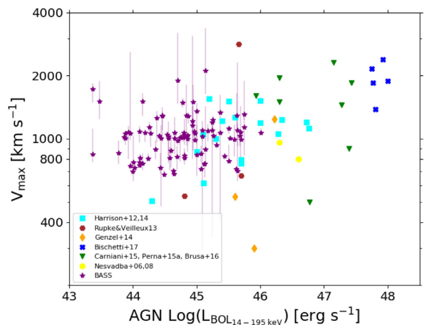
Figure 13. Maximum outflow velocities as a function of AGN \log(L_{\text{Bol}}) compared with several literature samples (Nesvadba et al. 2006, 2008; Harrison et al. 2012, 2014; Rupke & Veilleux 2013; Genzel et al. 2014; Carniani et al. 2015; Perna et al. 2015a; Brusa et al. 2016; Bischetti et al. 2017).
