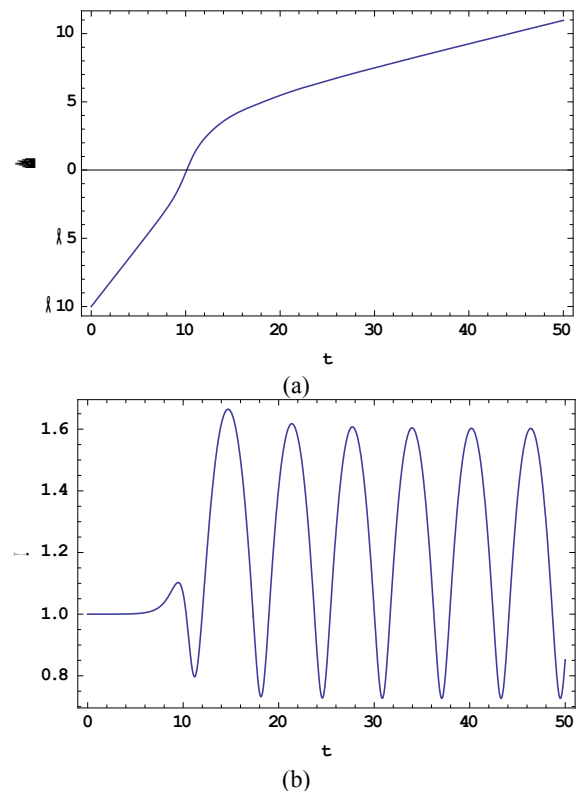
Fig. 3 Evolution of (a) center of mass position and (b) width of solitons in the presence of a Gaussian potential well at V_0 = 0.885 .
