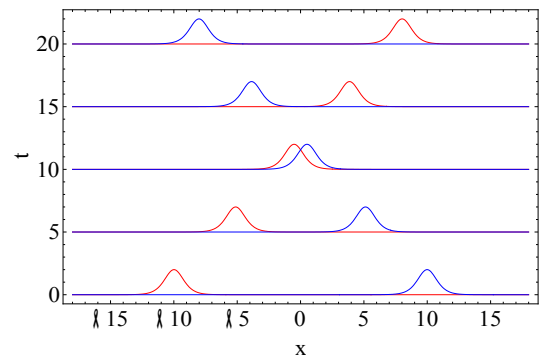
Fig. 2 Time evolution of vector solitons for V(x) = 0 and \beta = 0 .
