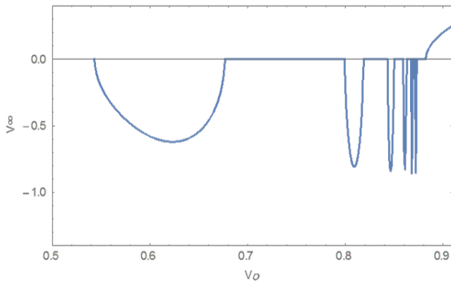
Fig. 7 The exit velocity versus collision velocity for ODE model Eqs. (14)-(15) at \beta = 0.2 .
