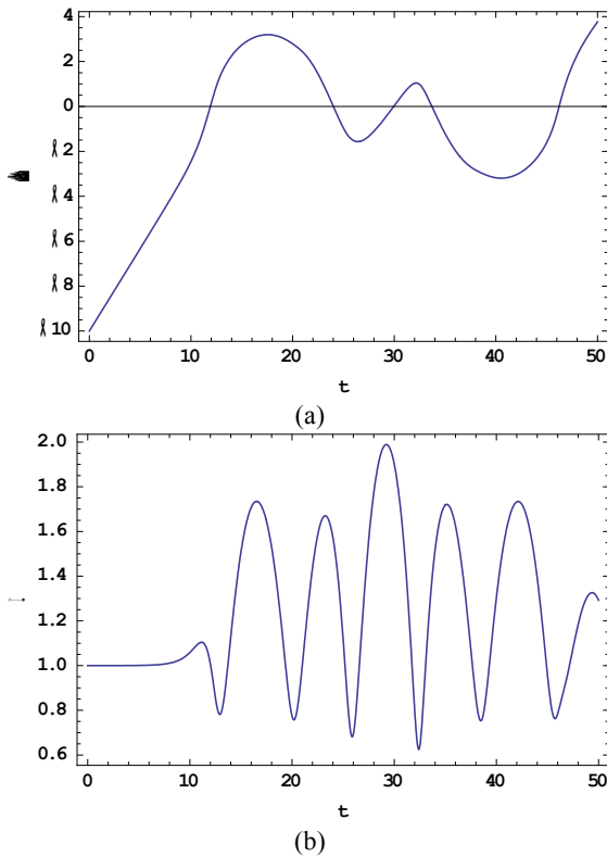
Fig. 4 Evolution of (a) center of mass position and (b) width of solitons in the presence of a Gaussian potential well at V_0 = 0.733 .
