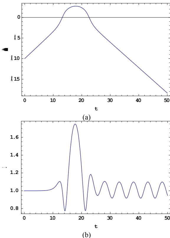
Fig. 5 Evolution of (a) center of mass position and (b) width of solitons in the presence of a Gaussian potential well at V_0 = 0.650 .
