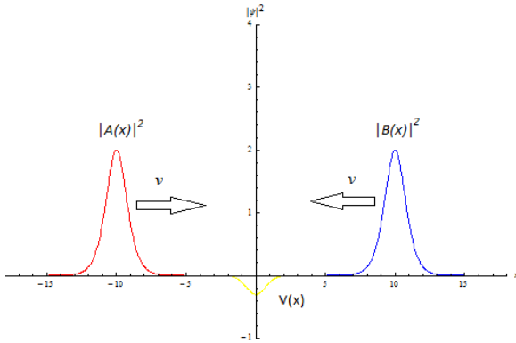
Fig. 1 Two solitons moving in different directions and scattering on the external potential V(x) .
