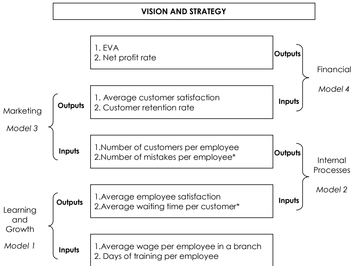
Figure 2 DEA Models
