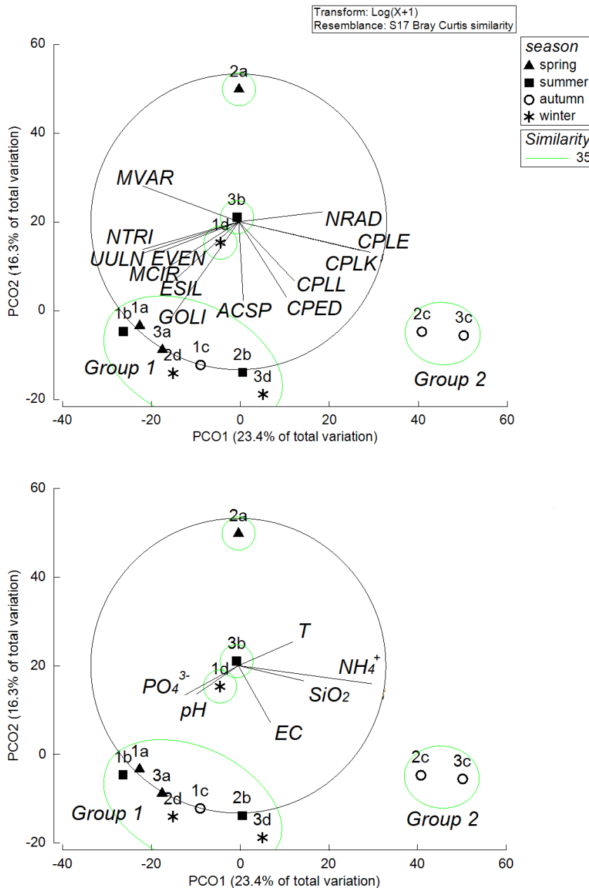
Fig. 3. Principal coordinates analysis (PCO) diagram comparing the community composition between samples in different seasons. PCO plot coded by the species vectors indicates taxa (A) and environmental vectors (B) positively correlated to PC1 and PC2 axes ( r > 0.5 ; r > 0.3 , respectively), and overlapped with the cluster groups based the 35% resemblance level of the group average clustering. Abbreviations: ACSP – Achnanthes sp., CPED – Cocconeis pediculus , CPLL – C. lineata , CPLK – C. placentula var. klinoraphis , CPLE – C. euglypta , MVAR – Melosira varians , EVEN – Encyonema ventricosum , ESIL – E. silesiacum , GOLI – Gomphonema olivaceum , MCIR – Meridion circulare , NRAD – Navicula radiosa , NTRI – N. tridentula , UULN – Ulnaria ulna ; T – temperature, \text{NH}_4^+ – ammonium, \text{SiO}_2 – silica, EC – conductivity, \text{PO}_4^{3-} – orthophosphate.
