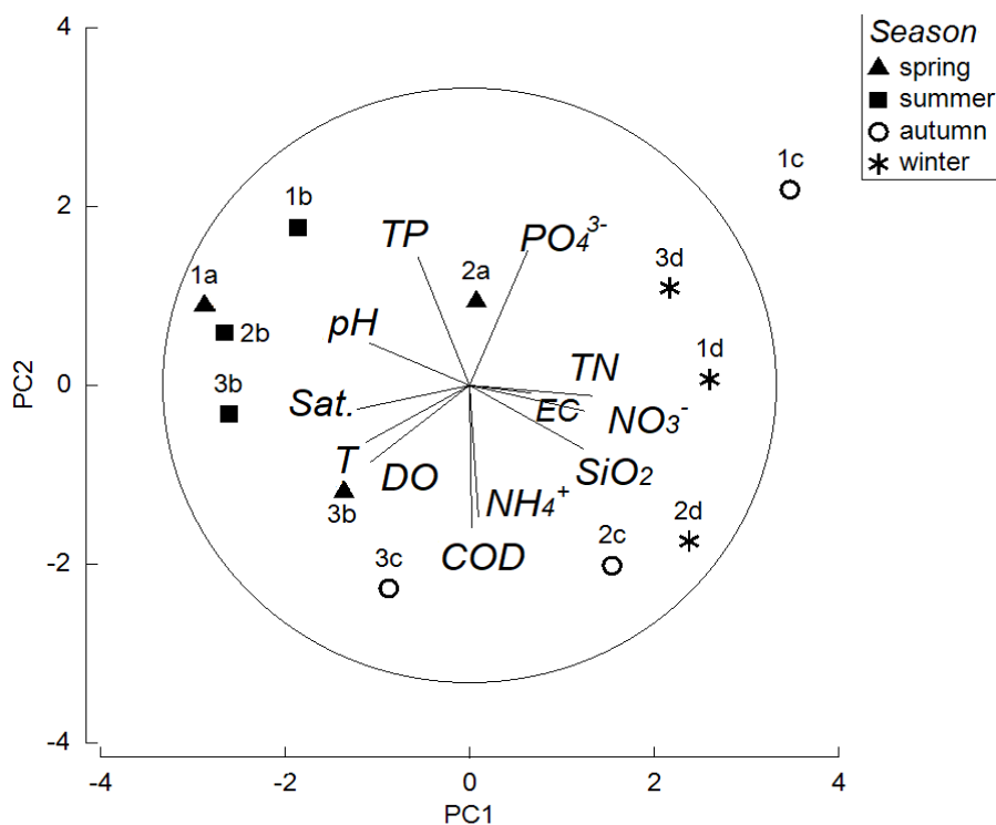
Fig. 2. Principal component analysis (PCA) ordination diagram performed on the environmental parameters for all sampling stations (1, 2, 3) in the Bunica River during four periods (a-spring, b-summer, c-autumn, d-winter) and overlapped with Pearson correlation vectors with PC1 and PC2 axes ( r > 0.4 ). Abbreviations: EC – conductivity, T – temperature, \text{NH}_4^+ – ammonium, \text{NO}_3^- – nitrate, TN – total nitrogen, \text{SiO}_2 – silica, \text{PO}_4^{3-} – orthophosphate, TP – total phosphorus, COD – chemical oxygen demand, DO – dissolved oxygen, Sat. – oxygen saturation.
