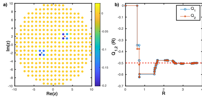
FIG. 5. (a) Density difference profile \rho(z_i) [see (19)] on a slightly disordered square lattice with the two quasihole coordinates, w_1 and w_2 , marked by the blue and the red star, respectively. The observation that \rho(z_i) is only nonzero in a finite region around each of the quasihole coordinates shows that the anyons are well screened. (b) The excess densities, Q_1 and Q_2 [see (18)], as a function of the radius R converge to the correct value -0.5 for a quasihole, which shows that the state is topological (see text). The number of lattice sites is N = 316 and the edge of the lattice is chosen to be roughly circular in order to resemble a quantum Hall droplet. The error bars due to Metropolis sampling are of order 10^{-4} .
