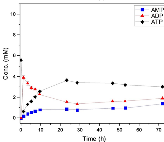
Figure 6. Time course of reaction products and intermediates for the synthesis of GDP-Fuc from Man, Guo, PolyP n , L-Glu, and catalytic amounts of ATP and NADPH. The experiments were carried out at 37 °C and 200 mM Tris-HCl (pH 8.5), 75 mM MgCl 2 , 10.5 mM Man, 10.5 mM Guo, 50 mM L-Glu, 1 mM NADPH, 5.5 mM ATP, 13.5 mM PolyP n , GSK (0.11 μg/μL), GMPK (0.49 μg/μL), PPK3 (0.02 μg/μL), GLK (0.33 μg/μL), MANB/C (0.17 μg/μL), WCAG (0.07 μg/μL), GMD (0.17 μg/μL), PPA (0.03 PPA), and 10 units of GLDH (2.99 μg/μL) in a final volume of 200 μL. The final DMSO content of the reaction matrix was 1% v/v. (a) shows the consumption of Guo, the production of GDP-Man and its consumption for synthesis of GDP-Fuc, (b) shows the production of GMP followed by its consumption for production of GDP and GTP, (c) shows the concentration of ATP, ADP as well as AMP; The production of AMP is mainly due to chemical conversion of ADP to ATP. Experiments were carried out in triplicates and error bars represent the standard error. The values of standard errors are listed in Table SI 3.
