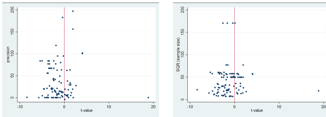
Figure 5.3: Funnel Plots for Precision and Size
