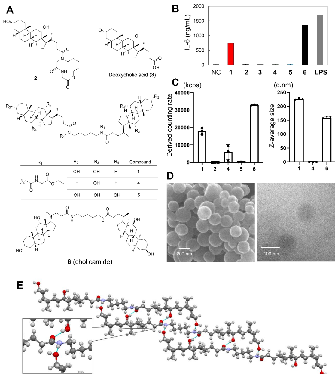
Fig. 3. Discovery of molecule 6 (cholicamide). (A) Chemical structures of molecules 1-6. (B) Effects of molecules 1-6 on the IL-6 production of RAW264.7 macrophages. All compounds were used at 30 \mu M. LPS was used at 100 ng/mL. NC = no compound. Error bar is the standard deviation ( n = 3 ). (C) Derived counting rate of molecules 1-6 and Z-average sizes of molecules 1, 4 and 6 as measured by DLS (Zetasizer Nano-s). (D) FE-SEM ( left ) and cryo-TEM ( right ) images of molecule 6 particles. (E) Interaction between two molecules of 6 in the crystal structure. Water molecules are omitted for clarity. Molecule 6 forms eight intermolecular hydrogen bonds with neighboring molecules (blue-dashed lines).
