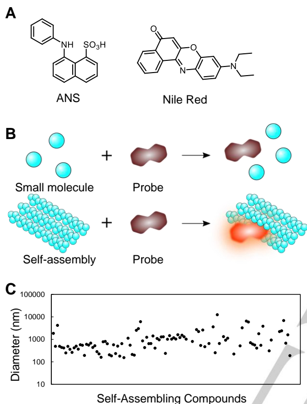
Fig. 1. Fluorescent-based screening for self-assembling molecules. (A) Chemical structures of ANS and Nile Red probes. (B) Illustration of the screening method. (C) Average hydrodynamic diameters of 116 self-assembling compounds as measured by DLS (ELS-Z2).
