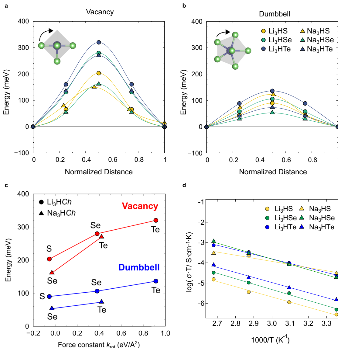
Fig. 5 Ionic conductivities of M_3HCh antiperovskites ( M = Li, Na , and Ch = S, Se, Te ). Low-barrier migration pathways for a vacancy and b interstitial dumbbell migration in M_3HCh . Top-left insets show M^+ migration when viewing HM_6 octahedron from the top to down. For orthorhombic Na_3HS , there are many migration pathways, one of which is shown as a representative example (see Supplementary Fig. 15 for details). c Migration barriers for cation transport via the vacancy and interstitial dumbbell mechanism in M_3HCh as a function of the force constant k_{rot} with respect to the HM_6 rotational motion. d Arrhenius plots of the total conductivity values for undoped M_3HCh cold-pressed samples in the temperature range from 25 to 100 °C.
