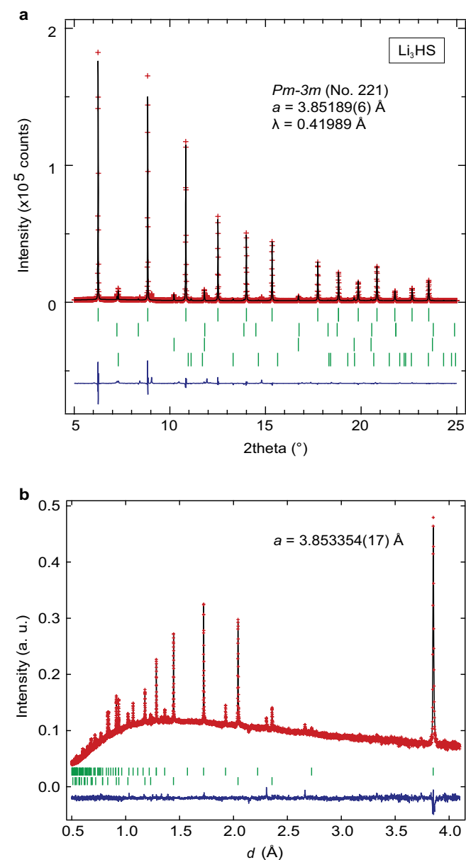
Fig. 2 Structural determination of \text{Li}_3\text{HS} . Rietveld refinement of a XRD and b ND. The red crosses, black solid line, blue solid line, and green dashes denote, respectively, the observed, calculated, difference intensities, and calculated Bragg reflections (from top to bottom: \text{Li}_3\text{HS} , \text{Li}_2\text{S} , \text{LiH} , BN in a ; \text{Li}_3\text{HS} , \text{LiH} in b ).
