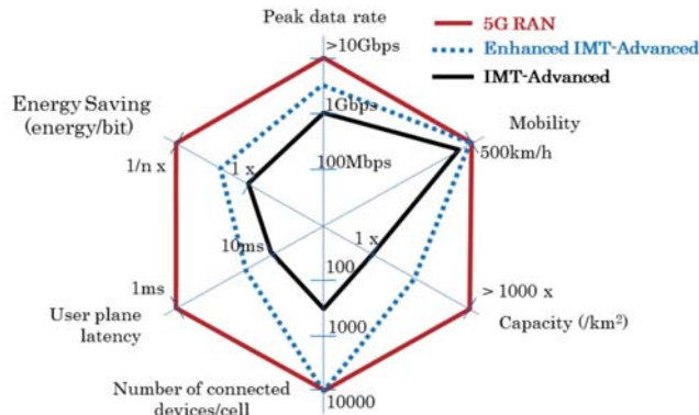
Fig. 1 Maximum system capabilities of 5G RAN [7].
