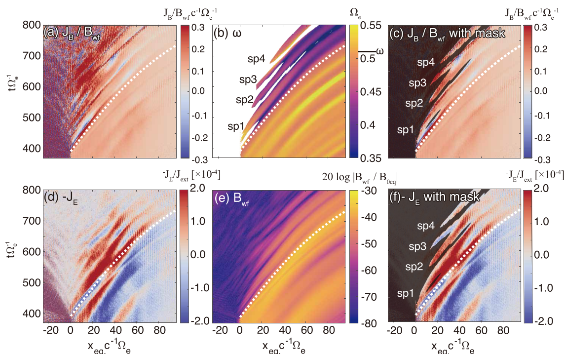
Figure 7. Falling-tone triggered wave packet from the Run 2 with the frequency of \omega = 0.51\Omega_e for (a) resonant current over magnetic field of forward wave J_B/B_{wf} , (b) wave frequency \omega , (c) J_B/B_{wf} for both conditions that the amplitude is more than -60 dB and that the magnitude-squared coherence at the local instantaneous frequency is more than 0.995, (d) resonant current -J_E , and (e) magnetic wave power \frac{1}{2}\mu_0 B_{wf}^2 . (f) -J_E by the same method as in (c).
