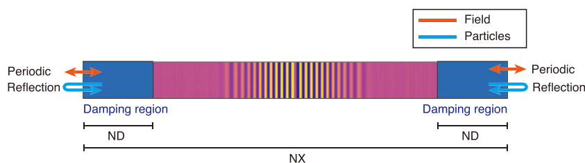
Figure 1. The schematic illustration of the one-dimensional simulation model. Total simulation region (NX) includes damping region (ND).
