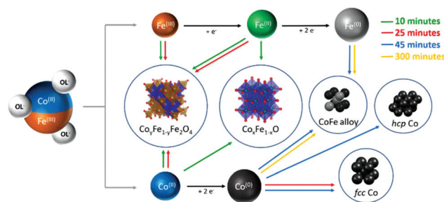
Scheme 1 Evolution of the composition of the final NHSs as a function of the dwelling time: the decomposition of the mixed \text{Co-Fe} precursor and the resulting reducing conditions lead to the simultaneous presence of metal atoms at different oxidation states, whose relative amount depends on the reaction time. Colored arrows indicate the phases found at different reaction times (green, red, blue and yellow correspond to 10, 25, 45 and 300 minutes, respectively).
