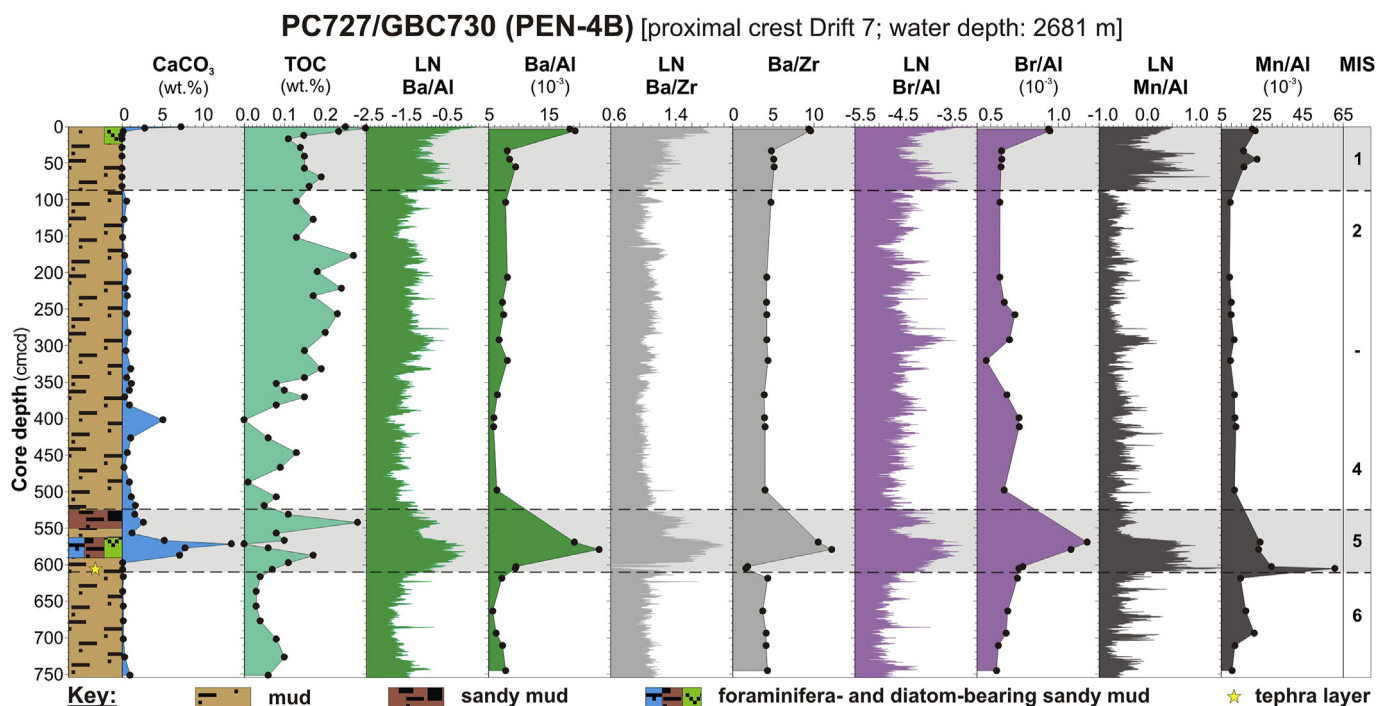
Fig. 12. Productivity proxies analysed on discrete samples (black dots) and with an XRF scanner in core PC727/GBC730. Mn/Al ratios are also shown.
