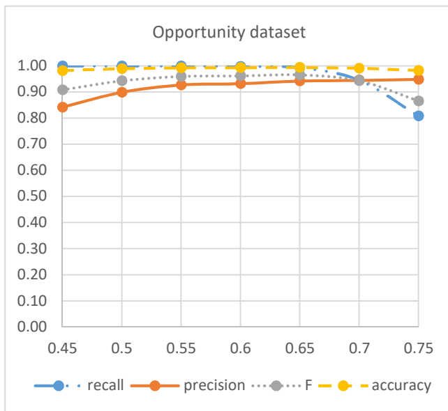
FIGURE 15. Detection of walking segments in the opportunity dataset
