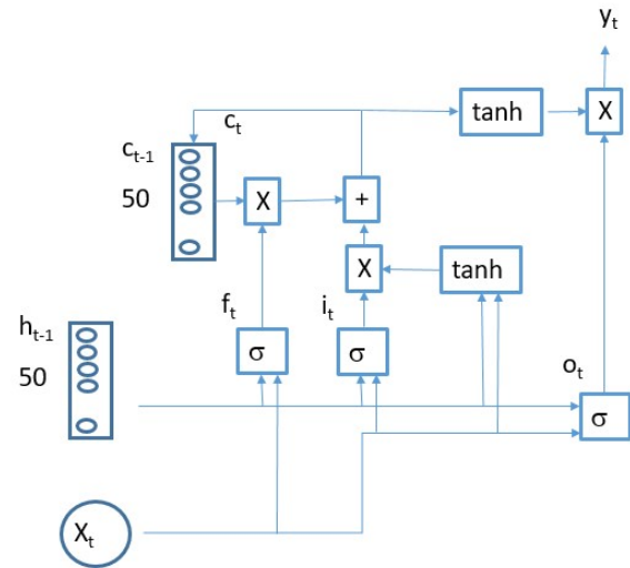
FIGURE 2. LSTM cell architecture.
