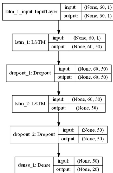
FIGURE 3. Graphical representation of the implemented model.
