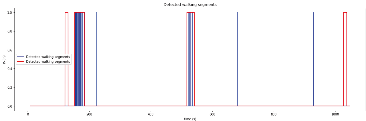
FIGURE 14. Detecting walking segments in a running recording
