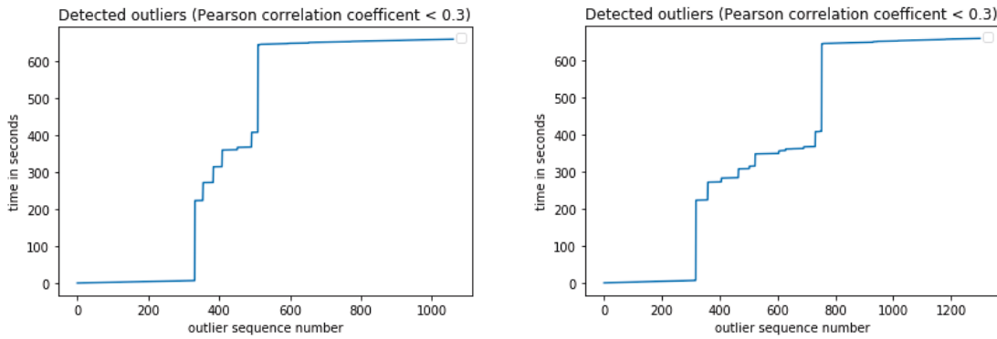
FIGURE 10. single and 2 iteration (outlier pre-filtering) outliers for participant 11.
