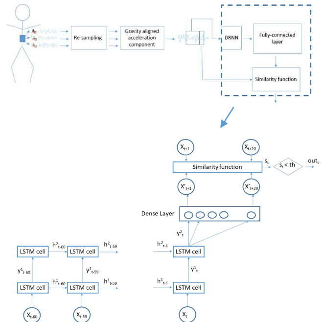
FIGURE 1. Proposed architecture.
