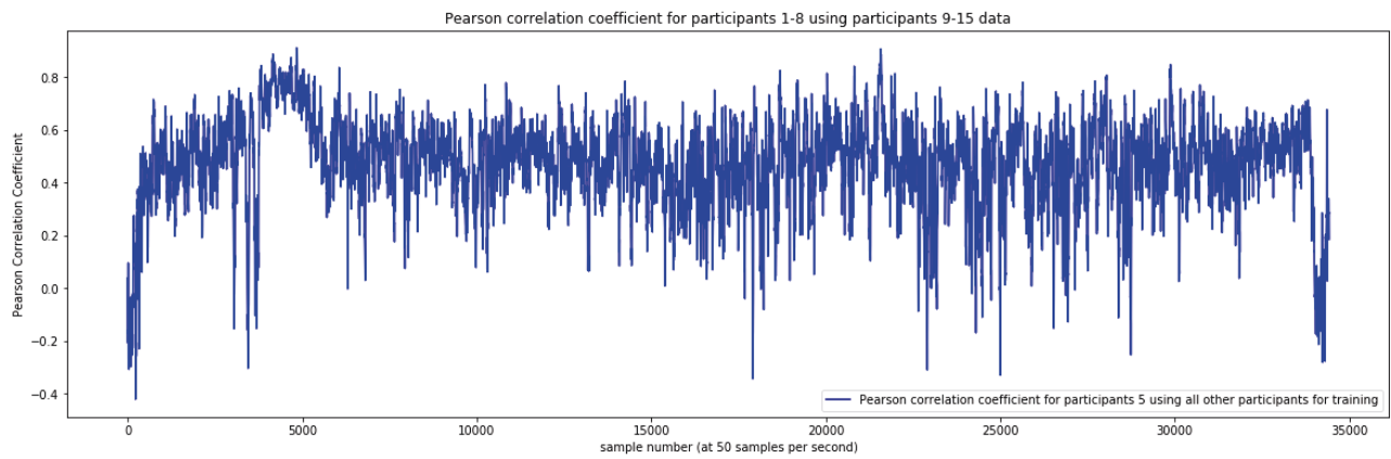
FIGURE 11. Similarities for participant 5 training with the rest of participants.
