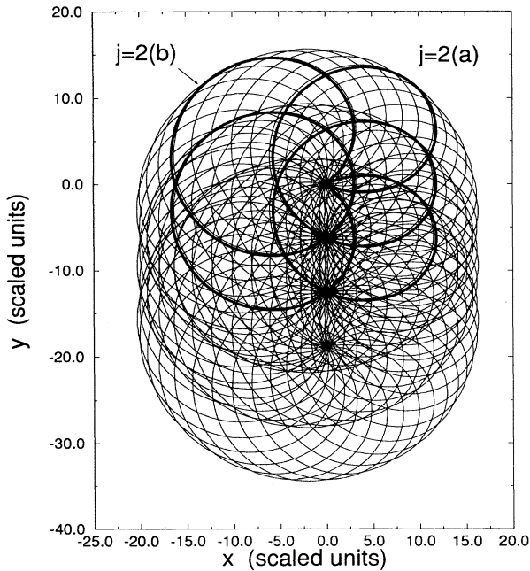
FIG. 9. For a scaled energy E=42 , above the second boundary energy, the second caustic has risen above the x axis. The “double-heart-shaped” orbit of Fig. 8 splits into two distinct orbits, and are associated with j=2(a) and 2(b) . We omit here the j=0 and 1 orbits.
