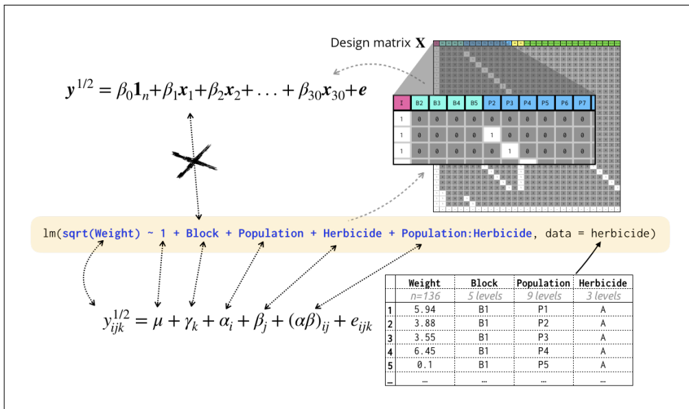
Figure 2: In the presence of categorical variables, the resemblance of the symbolic model formulae to its regression model form is not immediately obvious. In this case, categorical variables are transformed to a set of dummy variables with constraint applied for parameter identifiability. As such, a single categorical variable span a number of columns in the design matrix. On the other hand, if the model equation is written using the ANOVA model specification (with index notation), then the categorical variables have an immediate connection to the fixed effects in the model; see 2.2 for more information about the data and the model.
