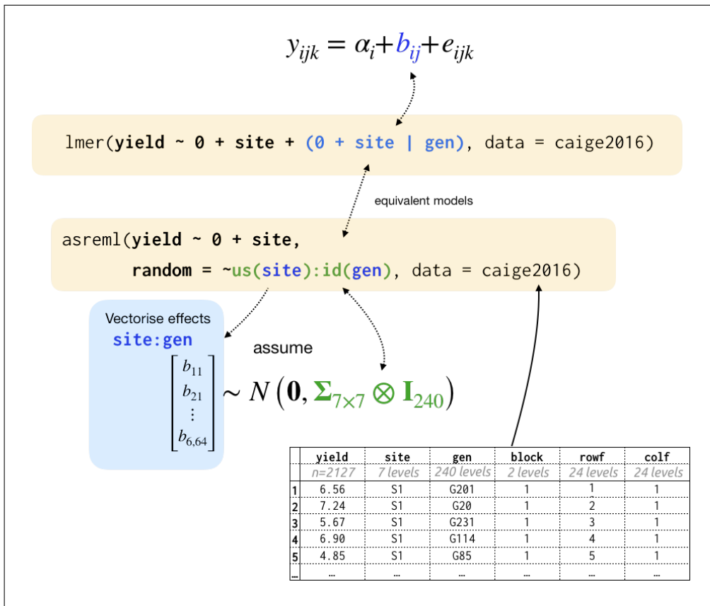
Figure 4: Depiction of the fit of a simplified LMM for the analysis of the MET data. In modelling the site-by-gen random effect, the variance structure are specified differently using lmer and asreml , where latter shows resemblances of covariance structure written mathematically and when all random effects are vectorised and concatenated, while the former requires some additional computation.
