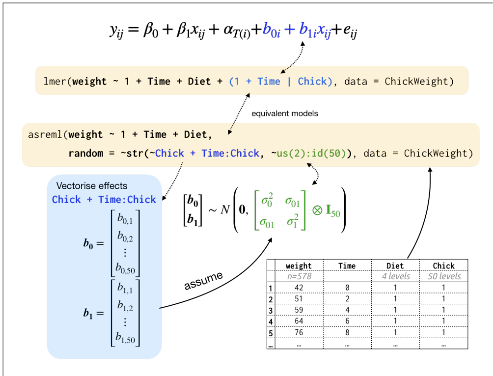
Figure 3: This figure shows a longitudinal analysis of the chicken data (see Section 4.1). The index form of the model equation shows direct resemblance for symbolic model formula in lmer for the fixed and random effects, however, its covariance form is not as easily inferred. In contrast, the symbolic model formula in asreml show resemblance of the covariance structure specified in the second argument of ~str , however, the corresponding random effects specified in the first argument of ~str must be vectorised as show in the above figure and requires implicit knowledge of the Kronecker product of relevant matrices.
