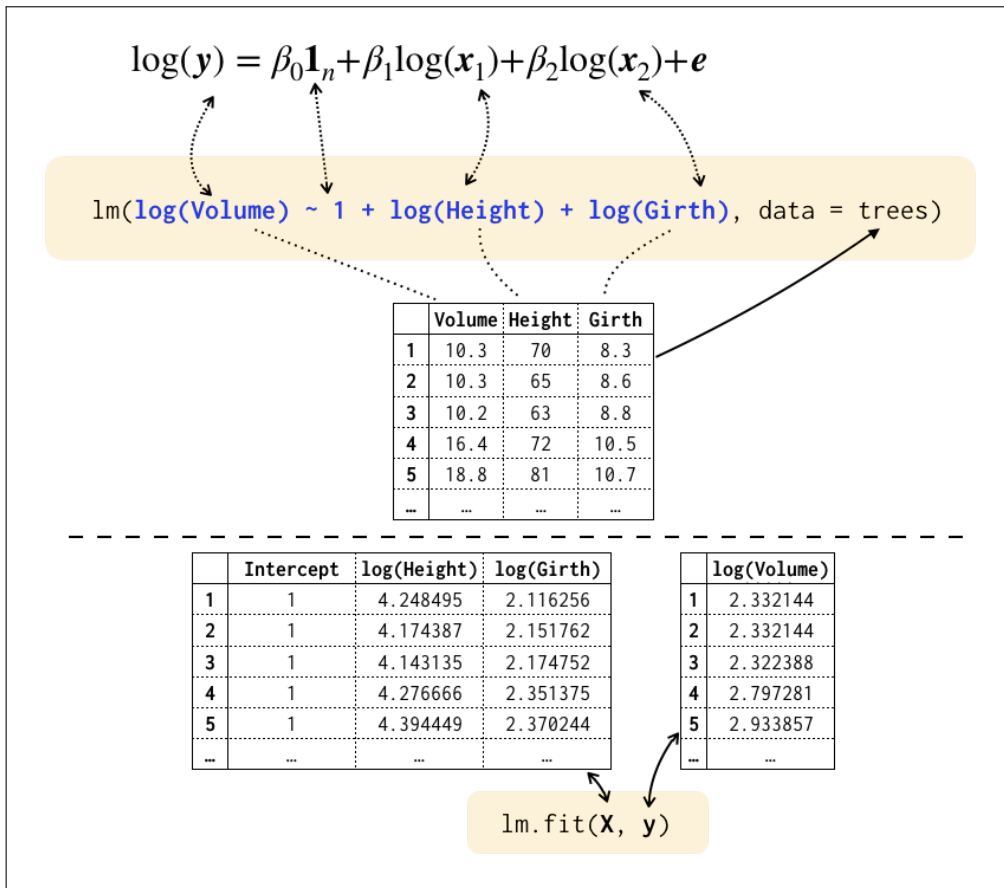
Figure 1: There are two main approaches to fitting a linear model illustrated above with the fit of a linear model to the trees dataset: (1) the top half uses the lm function with the input argument as a symbolic model formulae (in blue); (2) the bottom half uses the lm.fit function which requires input of design matrix and the response. The latter approach is not commonly used in R, however, it is the common approach in other languages; see Section 2.1 about the data and the model.
