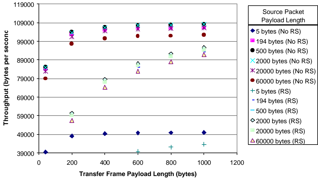
Figure 44. Throughput Variation With Transfer Frame Length In Graphical Format
