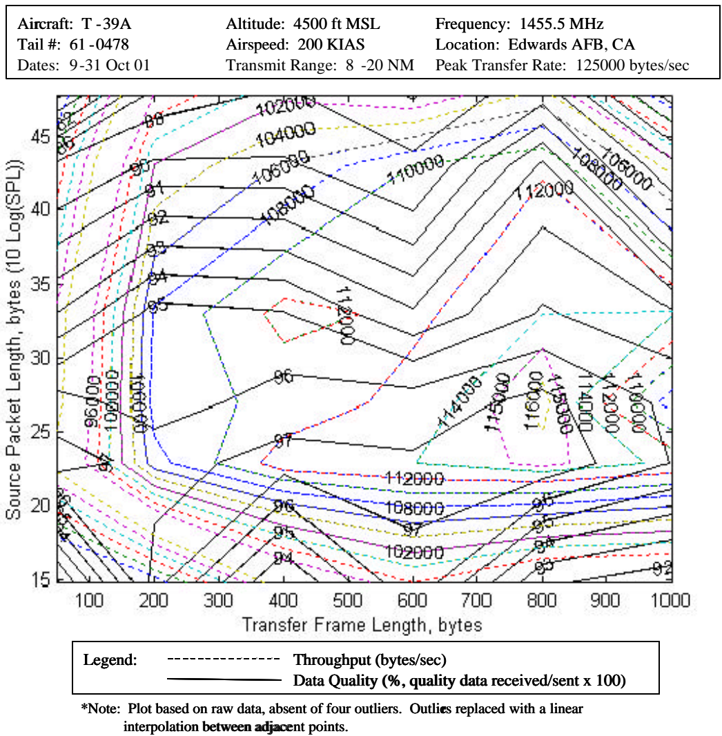
Figure 32: Contour Plot of Flight Test Data
