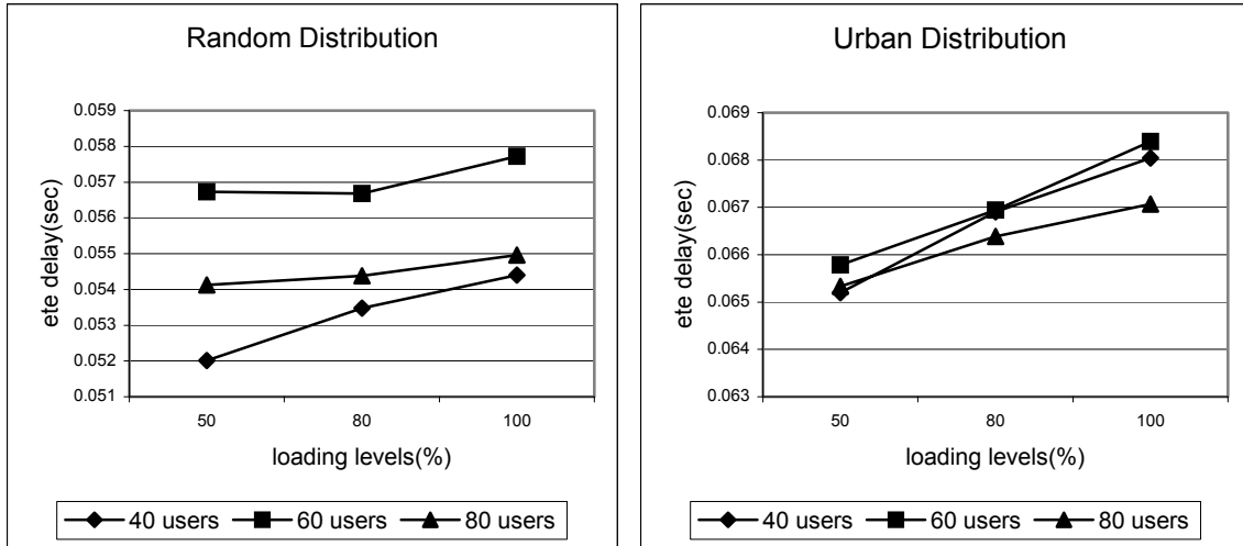
Figure 12 ODMRP End-to-End Delay In High Membership
