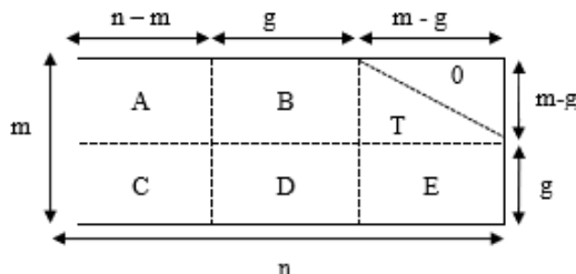
Fig. 1. Parity check matrix model [7]
