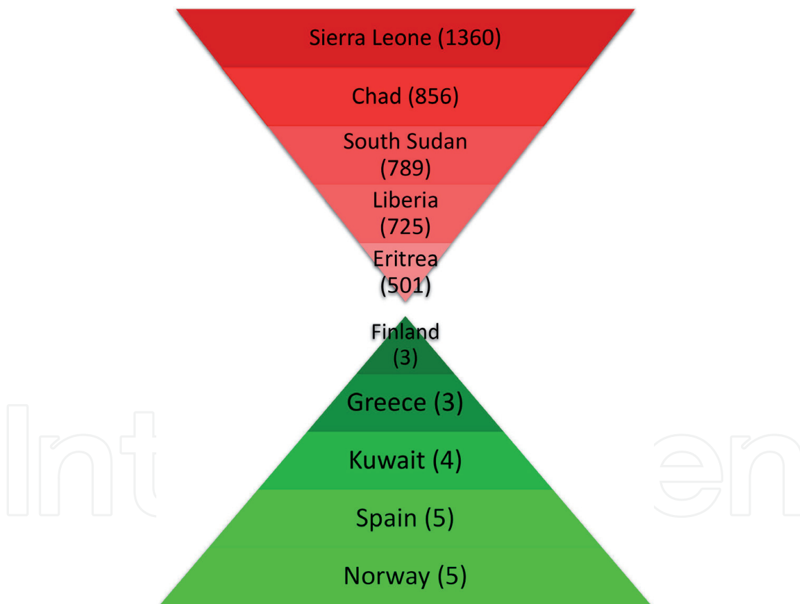
Figure 3. Sand clock of five countries with highest (red) and lowest (green) MMR.
