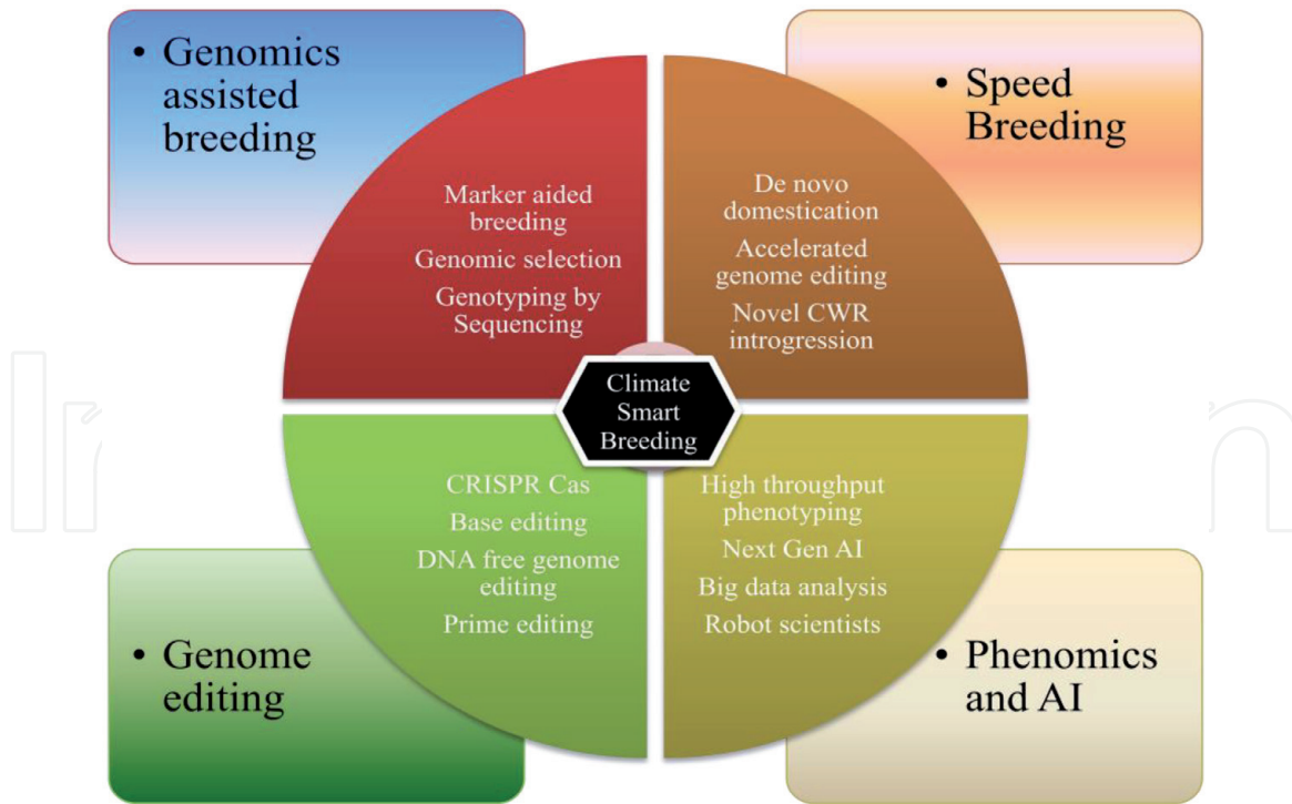
Figure 3. Compilation of state-of-the-art genomic, phenomic and computational tools comprising smart breeding approach for climatic resilience in agriculture.
